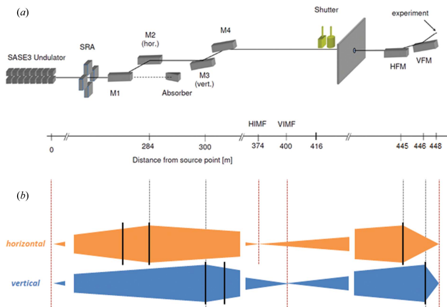
Figure 1 (a) Schematic representation of the beam transport layout of the SQS branch of the SASE3 beamline (Tschechschner et al. , 2017), which is described in detail in the text. The distance of each optical element to the source point is given at the bottom of the scheme. (b) The beam propagation conditions are schematically represented for both the vertical and the horizontal directions. The beam diverges from the source point until it reaches the first focusing element, which is M2 in the horizontal and M3 in the vertical direction. The beam converges horizontally and vertically on two different positions along the beamline, labeled HIMF and VIMF (horizontal and vertical intermediate focus, respectively), located at 90 m and 100 m distance from the respective mirrors. These positions are then the virtual sources imaged by the HFM (horizontal focusing mirror) and VFM (vertical focusing mirror) into the focal position where the experiment takes place. The dashed vertical lines indicate the position of the focusing mirrors and of the (virtual) sources and images in the vertical and horizontal directions.
