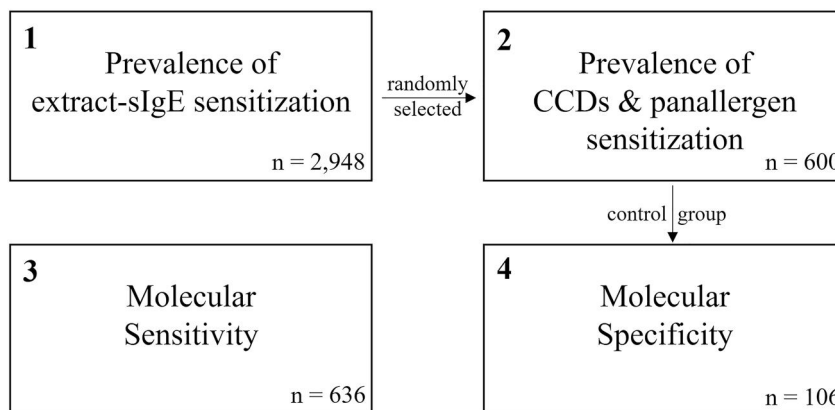
FIGURE 1 Flow-chart of the four analyses performed. In total, clinical data and test results of 3,590 patients were investigated. Patients of analysis 2 were randomly selected from analysis 1 ( 6 \times 100 patients with 0–5 pollen sensitizations). The control group from analysis 2 (100 patients without pollen allergy) and six additional patients were used for analysis 4.
