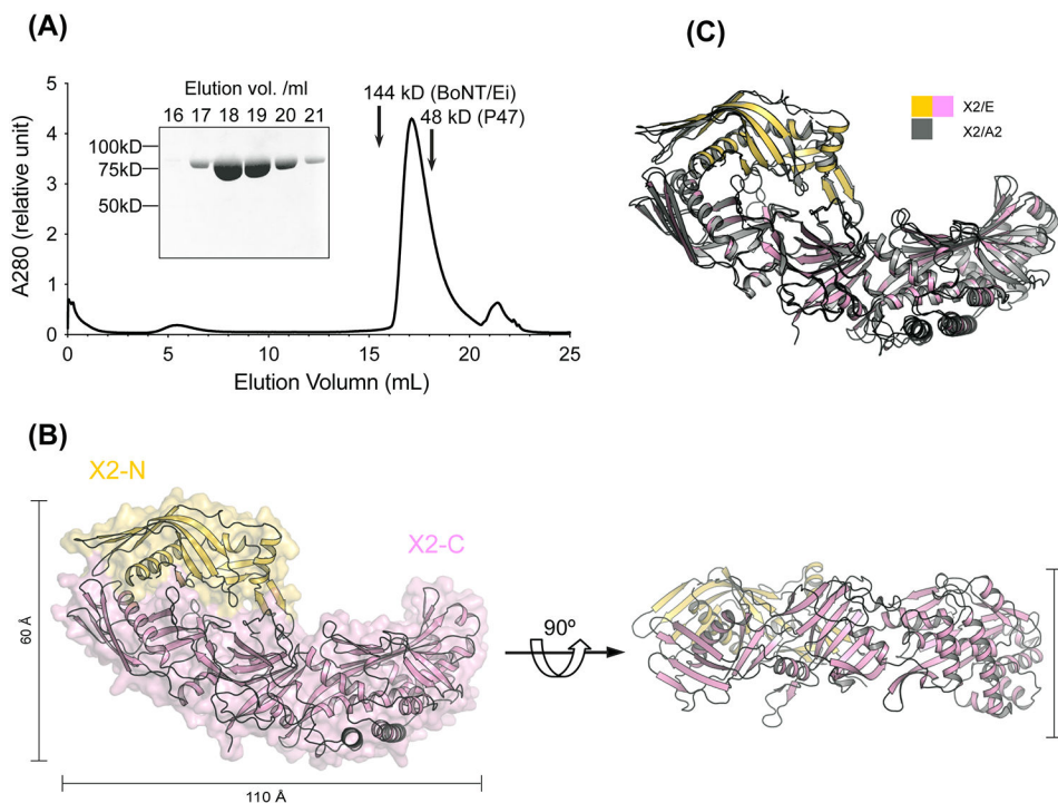
Figure 4. Crystal structure of BoNT/E OrfX2.
