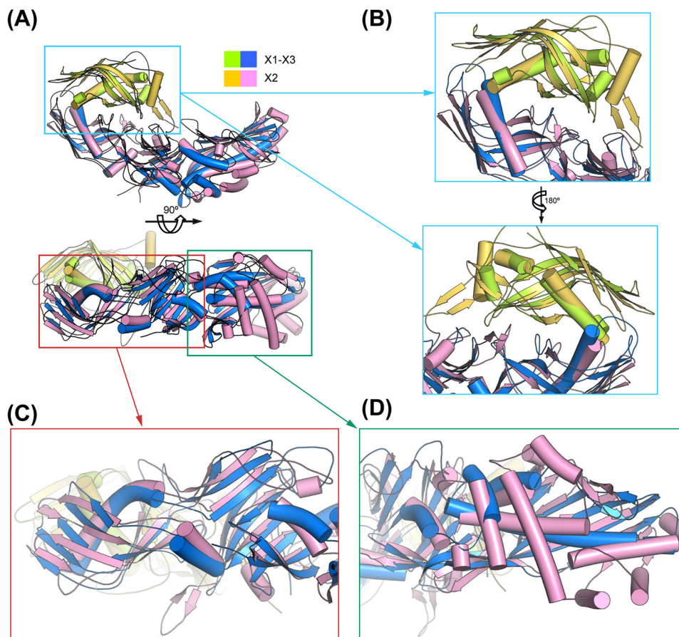
Figure 5. Structural comparison between the OrfX1–OrfX3 complex and OrfX2. (A) Superimposition of the OrfX1 (lime green)–OrfX3 (blue) complex and OrfX2 (yellow and pink). (B) Close-up views of the superimposed OrfX1–OrfX3 interface and OrfX2–N–OrfX2–C interface. (C–D) Close-up views of the superimposed OrfX3 and OrfX2–C focusing on the N-terminal TULIP-like domain and the connecting central \beta -sheet (C) and the C-terminal TULIP-like domain (D).
