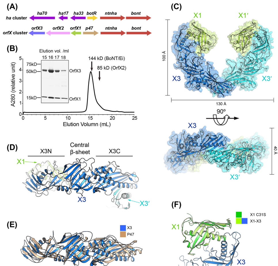
Figure 1. Crystal structure of the tetrameric OrfX1-OrfX3 complex.
