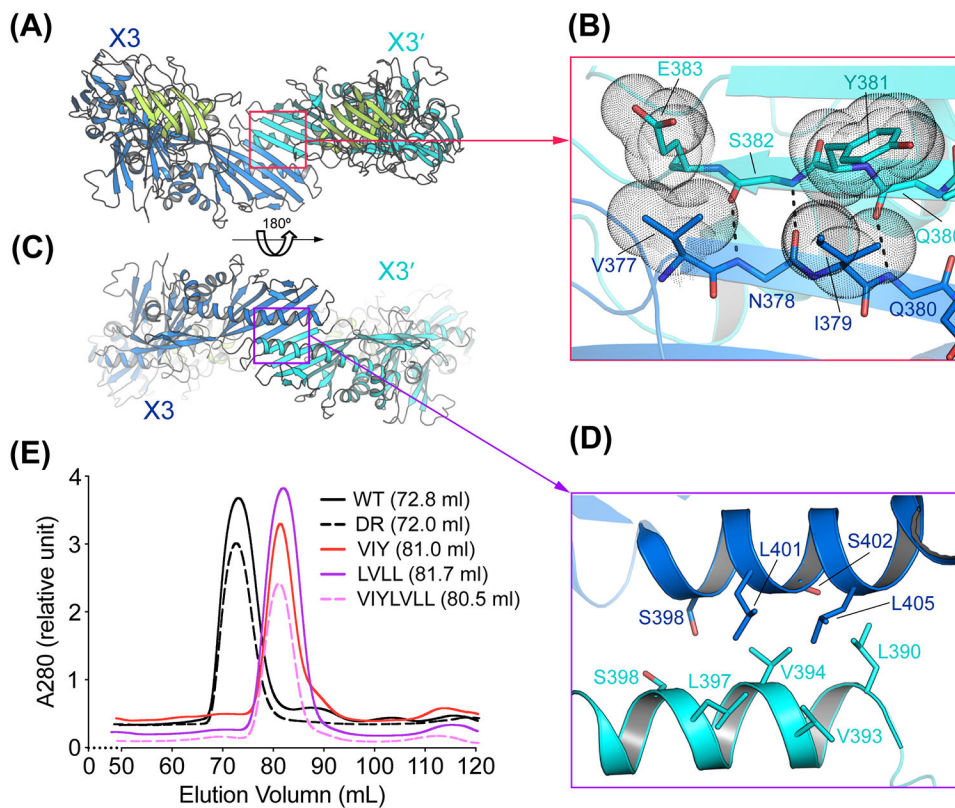
Figure 3. Interactions between the homodimeric OrfX3 in the OrfX1-OrfX3 complex. (A, C) Two different views of the OrfX1-OrfX3 complex focusing on the OrfX3 dimer interface. (B, D) Close-up views of key interacting residues around the antiparallel edge-to-edge \beta -strand interface between the two OrfX3-C units (B) and the interface between the long \alpha -helix from each OrfX3-C domain (D). Hydrogen bonds are shown as dashed lines. Residues V377, I379, Y381 that were subjected for mutagenesis study and E383 are shown as dotted spheres. Please note that another set of homodimeric OrfX3 interactions related to that shown in panels B and D by a \sim 180^\circ rotational symmetry are not shown for clear illustration. (E) The WT (n=3) and four mutant OrfX1-OrfX3 complexes (n=1) were analyzed by size exclusion chromatography using a Superdex-200 16/60PG column with peak retention volumes indicated.
