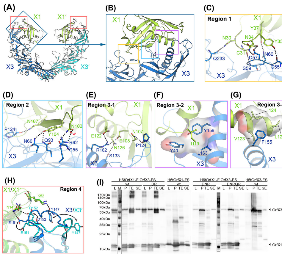
Figure 2. Interactions between OrfX1 and OrfX3.
