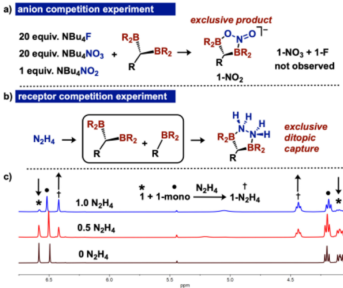
Figure 4. Anion competition reaction showing selective nitrite capture by 1 in the presence of fluoride and nitrate (top), selectivity of hydrazine binding to 1 in the presence of 1-mono (middle) and ^1\text{H} NMR of hydrazine competition experiment (bottom) ( \text{N}-\text{CH}_2 and \text{pyz}-\text{CH} shown). \text{BR}_2 = 9\text{-BBN} and \text{R} represents the remainder of the free ligand.
