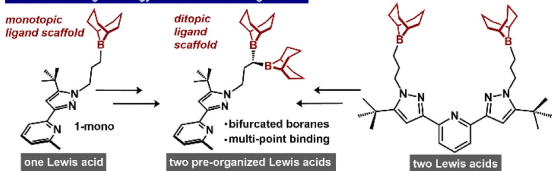
Figure 1. Selected examples of known ditopic boranes, [11, 12b, 14, 15e] and design strategy outlining the ditopic ligand used in this work from prior work using a bidentate ligand with single second-sphere Lewis acid, [9a-c] and a tridentate ligand with two Lewis acids, [4, 9d, 9e]
