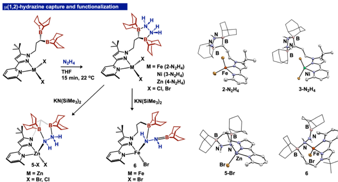
Figure 5. \mu(1,2) -hydrazine capture using 2–4 to yield 2–4-N 2 H 4 and hydrazine reactivity of 2-N 2 H 4 and 4-N 2 H 4 to generate hydrazido and diazene complexes 5-X and 6 (X = Br, Cl). Molecular structures of 2-N 2 H 4 , 3-N 2 H 4 , 5-Br and 6 (right). Thermal ellipsoids displayed at 50% probability. Non-diazeno or hydrazine H-atoms are omitted, and the 9-BBN substituents are displayed in wireframe for improved clarity.
