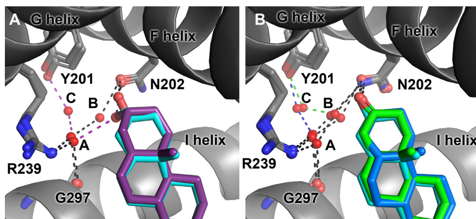
Figure 3. Abiraterone metabolites with modifications of the A ring participate in different hydrogen bond networks. A, the 3 \beta -OH of abiraterone (cyan, from PDB 3RUK) hydrogen bonds directly to N202, while the abiraterone analog 3 \alpha -OH (purple) instead directly interacts with water A, which in turn is within a distance to interact with R239, G297, and water C. Water C bridges to Y201 for the 3 \alpha -OH complex but is not apparent in the abiraterone structure. B, like abiraterone (cyan, from PDB 3RUK), abiraterone 3-keto, \Delta 4 (blue), and 3-keto, 5 \alpha (green) analogs both form a hydrogen bond directly to N202, and this residue further engages in a hydrogen bonding network via two water molecules (A and B) bridging to R239 and the backbone carbonyl of G297. However, like the 3 \alpha -OH analog, a third water molecule (C) forms interactions with Y201 in the F helix. PDB, Protein Data Bank.
