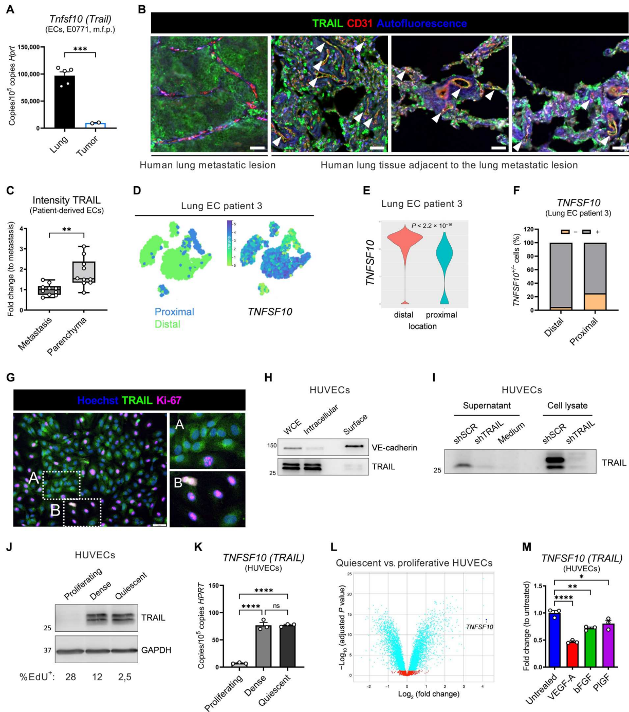
Fig. 4. TRAIL expression is a trait of EC quiescence. (A) mRNA expression of Tnfsf10 in ECs sorted from perfused lungs or primary tumors of E0771 tumor-bearing WT mice (day 14). (B and C) Histological analysis of vasculature (CD31; red), TRAIL (green), and autofluorescence (blue) in a metastatic lesion or its adjacent parenchymal tissue in postmortem lung samples from two patients with breast cancer. Dots in (C) represent the average intensity in 10 different fields (5 fields per patient). Arrowheads in (B) show colocalization of CD31 and TRAIL (yellow). Scale bars, 50 \mu m. (D to F) t-SNE plots showing the origin (distal versus proximal) or expression of indicated genes (D), violin plot showing expression levels (E), or the percentage of expressing (+) and nonexpressing (–) cells (F) in ECs from patient 3. (G) Immunofluorescence costaining of TRAIL (green), Ki-67 (magenta), and Hoechst (blue). Higher-resolution inset of confluent (A) or proliferative (Ki-67 + ) areas (B). Scale bar, 50 \mu m. (H to J) Protein levels of TRAIL in whole-cell extract (WCE), intracellular, or surface fractions of quiescent HUVECs (H); in supernatant protein precipitates or WCE of quiescent HUVECs treated with the pan-caspase inhibitor q-VD-OPh (qVD) (50 \mu M) for 18 hours (I); or in proliferating, dense, or quiescent HUVECs (5-ethynyl-2'-deoxyuridine, EdU) (J). In (H), VE-cadherin is the representative surface protein. (K) mRNA expression of TNFSF10 in proliferating, dense, or quiescent HUVECs. (L) Volcano plot showing TNFSF10 transcript distribution. Positive and negative log 2 (fold change) values (x axis) represent up-regulation or down-regulation, respectively, in quiescent compared to proliferative HUVECs. Dots in blue represent significant differentially expressed genes. (M) mRNA expression of TNFSF10 in quiescent HUVECs treated with VEGF-A (50 ng/ml), bFGF (10 ng/ml), or PIGF-1 (50 ng/ml) for 17 hours. All graphs show means \pm SEM. * P < 0.05 ; ** P < 0.01 ; *** P < 0.001 ; **** P < 0.0001 .
