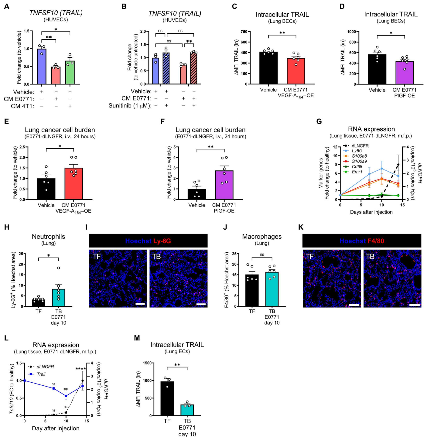
Fig. 5. TRAIL expression is down-regulated by tumor-derived factors during PMN formation. (A and B) mRNA expression of TNFSF10 in HUVECs treated for 24 hours with a conditioned medium (CM) of E0771 or 4T1 cancer cells for 48 hours and/or with sunitinib (1 \mu M). (C and D) FACS analysis of intracellular TRAIL protein in lung ECs from WT mice injected 12 times i.v. with a CM of E0771 cells overexpressing (OE) murine VEGF-A 164 (C) or PIGF (D) for 48 hours. \Delta MFI = MFI stained - MFI isotype . (E and F) mRNA expression of dLNGFR in perfused lung tissue 24 hours after i.v. injection of E0771-dLNGFR in WT mice injected 12 times i.v. with a CM of E0771 cells overexpressing VEGF-A 164 (E) or PIGF (F) for 48 hours. Vehicle represents a mock medium, pseudo-conditioned in absence of cancer cells. (G) mRNA expression of Ly6g , S100a8 , S100a9 , Cd68 , Emr1 , and dLNGFR in perfused lung tissue from WT mice after orthotopic m.f.p. injection of E0771-dLNGFR cells. (H to K) Histological analysis of Ly-6G + neutrophil area (H and I) and F4/80 + macrophage area (J and K) in tumor-free (TF) WT mice or tumor-bearing (TB) WT mice 10 days after orthotopic m.f.p. injection of E0771-dLNGFR cells. Scale bars, 50 \mu m. (L) mRNA expression of Tnfsf10 and dLNGFR in perfused lung tissue from WT mice after orthotopic m.f.p. injection of E0771-dLNGFR cells. FC, fold change. (M) FACS analysis of intracellular TRAIL protein in lung ECs from tumor-free WT mice or 10 days after orthotopic m.f.p. injection of E0771-dLNGFR cells. \Delta MFI = MFI stained - MFI isotype . All graphs show means \pm SEM. * P < 0.05; ** P < 0.01; ### P < 0.01; **** P < 0.0001.
