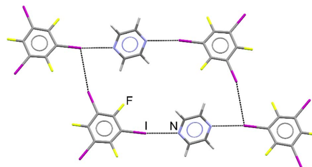
Fig. 1 Structure of the cocrystal of pyrazine with 1,3,5-trifluoro-2,4,6-triiodobenzene, further labelled as ( pyr ) 1/2 ( tftib ). Intermolecular N \cdots I and I \cdots I interactions are shown.
