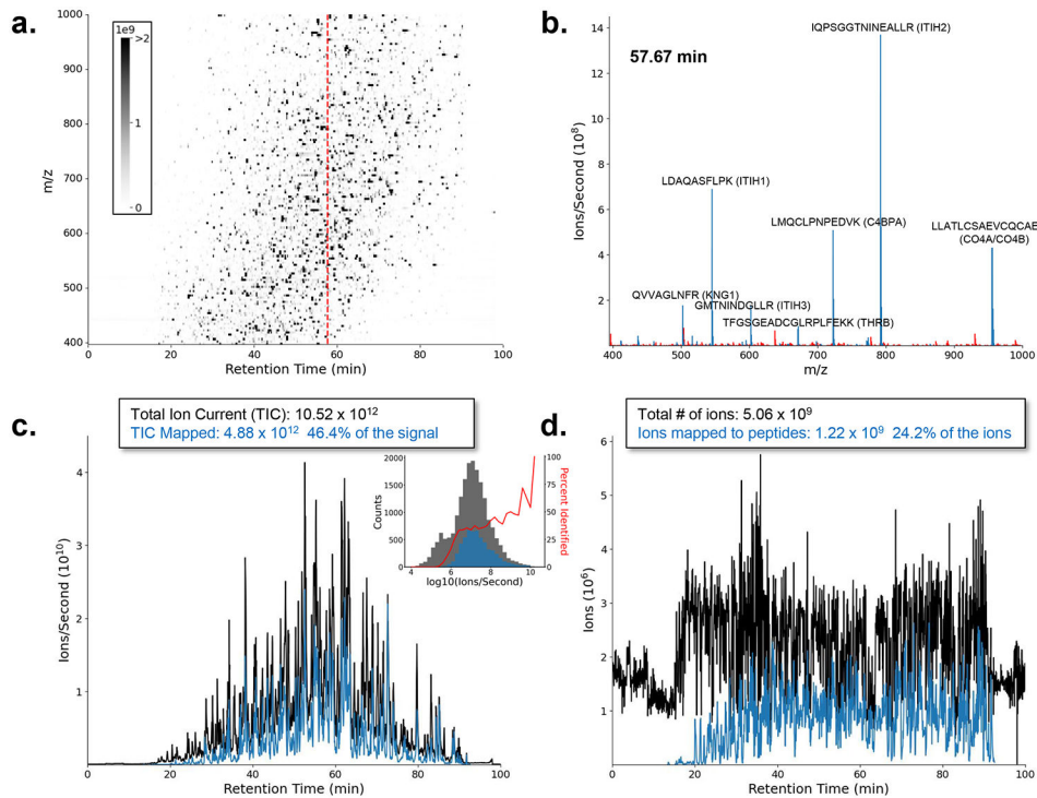
Figure 2 | A liquid chromatography-mass spectrometry experiment can count billions of peptide ions within 90 min.
