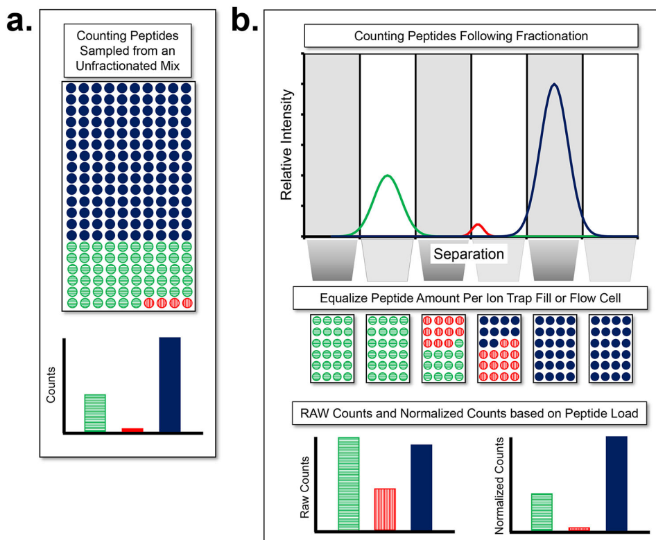
Figure 3 | Fractionation prior to counting molecules improves the dynamic range in proteomics.
