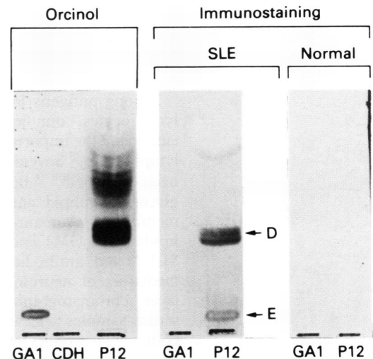
Figure 4 Thin layer chromatography of neutral glycosphingolipids from P12 cells with a serum sample from a patient with SLE and a normal control subject. The neutral glycosphingolipids from P12 cells and asialoGM1 are abbreviated to P12 and GA1 respectively. The left hand plate was stained with orcinol- H_2SO_4 reagent. The right hand plate was immunostained with serum samples from the patient with the lowest lymphocyte count and a normal control subject. Neutral glycosphingolipids D and E were stained with a serum sample from the patient, but not the normal control subject. CDH=ceramide dihexosides.
