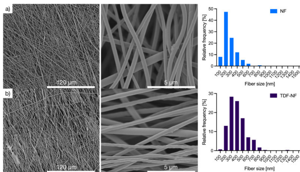
Figure 15. Representative SEM (scanning electron microscope) images and fiber size distributions ( n = 300 ) of (a) drug-free nanofibrous mat (NF) and (b) tenofovir disoproxil fumarate-loaded nanofibrous mat (TDF-NF) prepared with CS and PEO at a ratio of 1:4 ( w/w ). SEM images magnifications: \times 1000 and \times 10,000 [258]. Reproduced with permission from Elsevier (Copyright © 2022).
