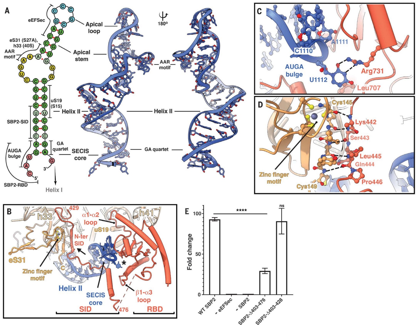
Fig. 3. Human SBP2•SECIS captured on the translating ribosome.
