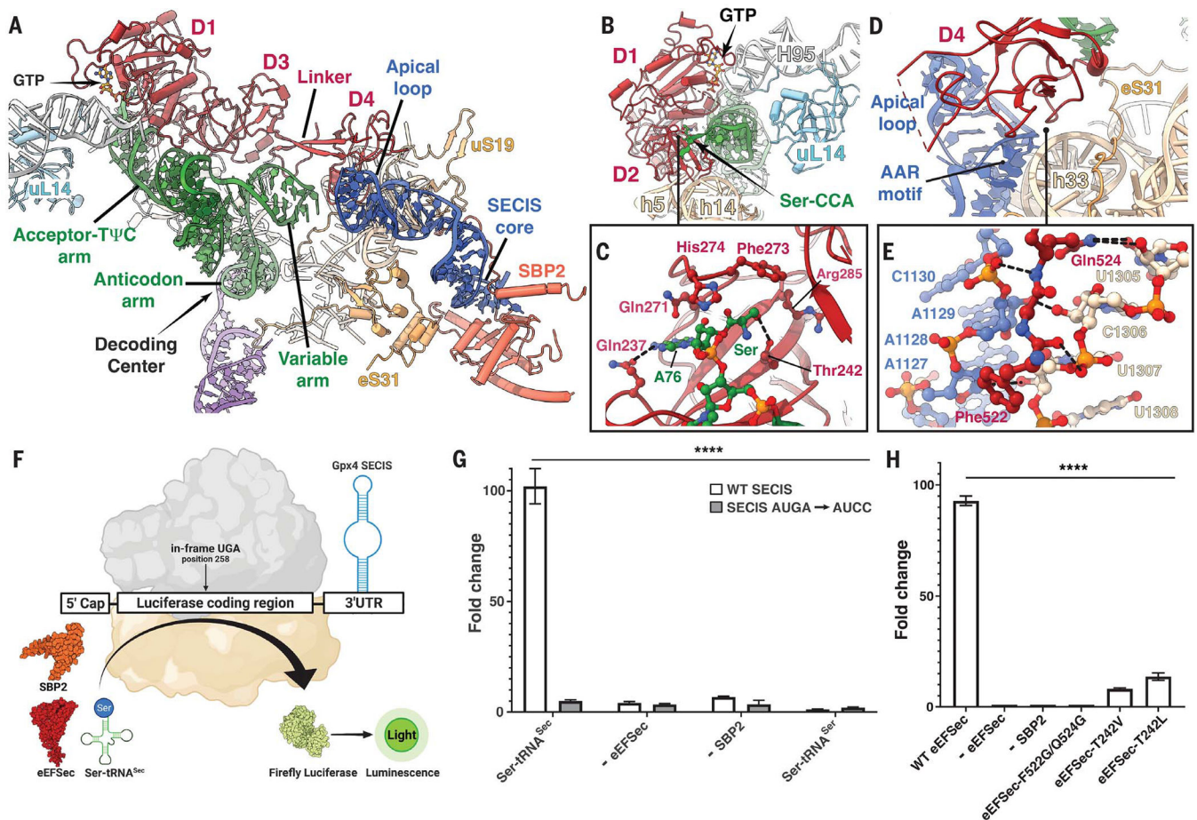
Fig. 2. Human eEFSec•GTP•Ser-tRNA Sec on the 80S ribosome.
