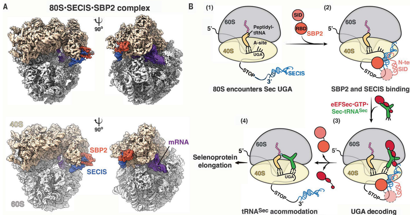
Fig. 4. Eukaryotic selenoprotein elongation at Sec UGA codons.
