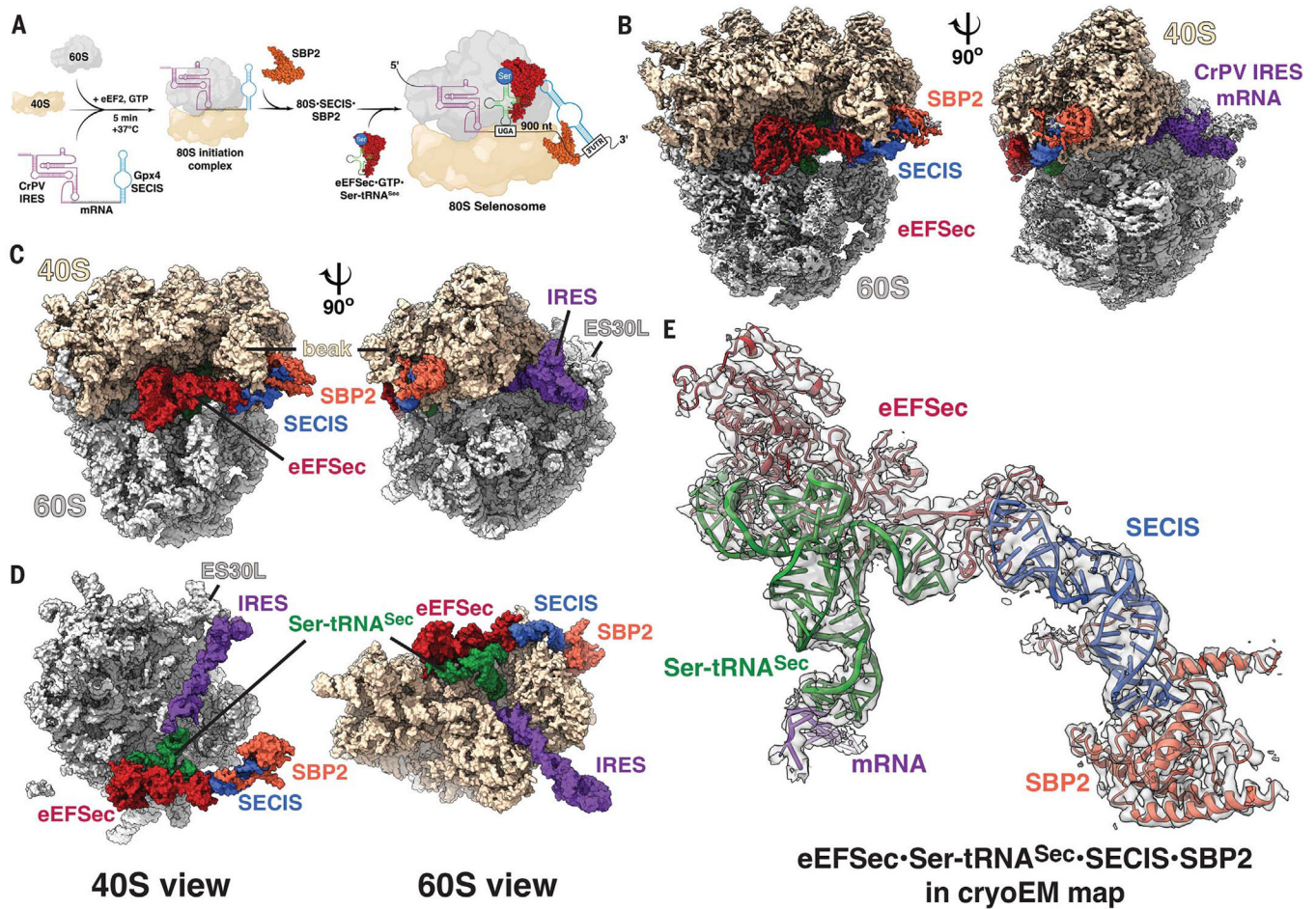
Fig. 1. The mammalian Sec UGA recoding assembly.
