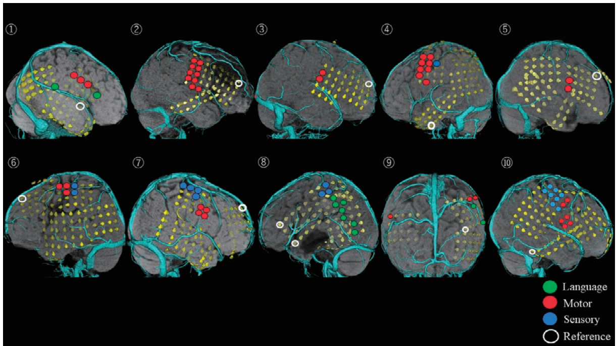
Fig. 1 The locations of electrodes and eloquent cortices in Pt. 1-10. The green, red and blue circles indicate the electrodes that elicited the language, motor and sensory symptoms in the monopolar functional mapping, respectively. The white circles indicate the reference electrodes in monopolar cortical stimulation.
