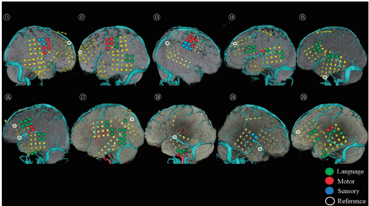
Fig. 2 The locations of electrodes and eloquent cortices in Pt. 11-20.
