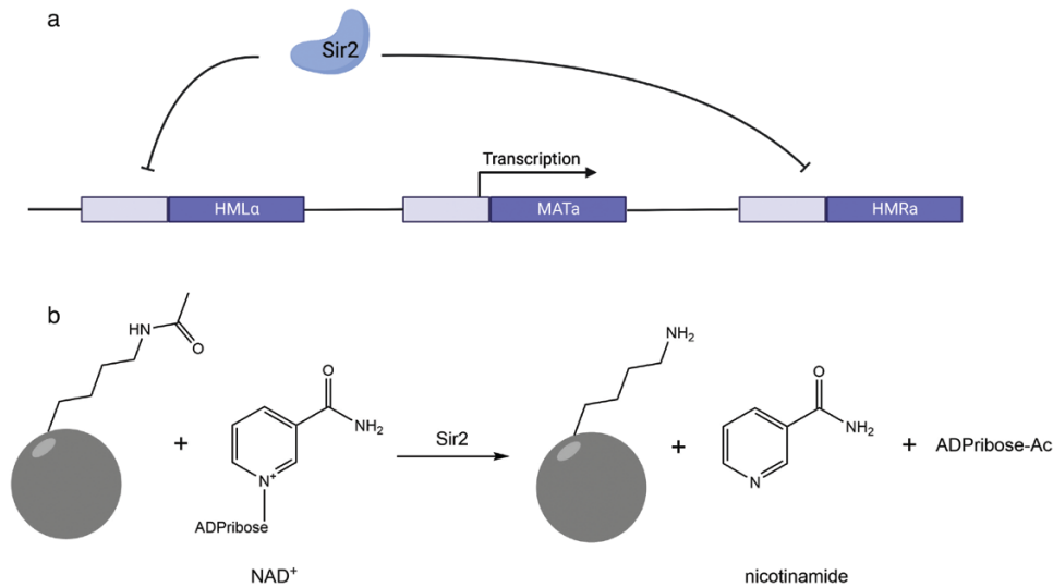
Figure 1 Sir2 enzymes are gene silencers in fungi and are conserved as NAD + -dependent protein lysine deacylases. (a) In Saccharomyces cerevisiae , the SIR2 gene is required to silence genes in particular chromosomal locations. This function is to be conserved across divergent yeasts. (b) The biochemical function of sirtuins is largely conserved. These enzymes deacetylate protein lysine substrates in a manner that depends on NAD + , which produces the deacetylated protein lysine substrate, nicotinamide, and acylated ADPribose.
