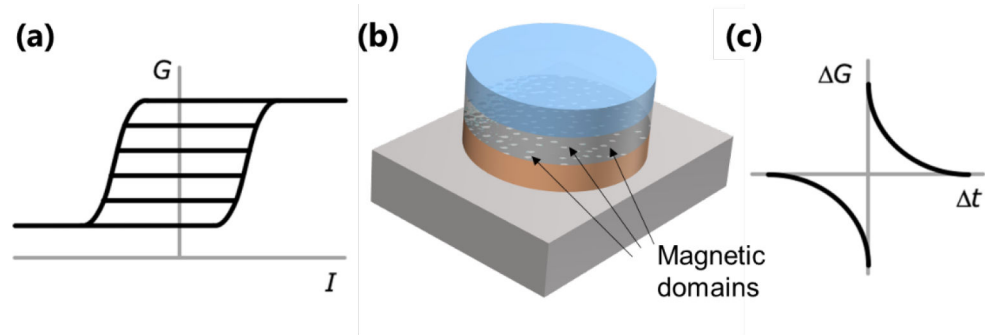
Figure 14. Functions of SOT memristor. (a) Conductance G versus current I of analog memory. (b) Snapshot of fine ferromagnetic domains in an antiferromagnet/ferromagnet system. (c) Conductance change \Delta G versus timing difference between firing of post and pre neurons \Delta t for spike-timing-dependent plasticity (STDP) synapse.
