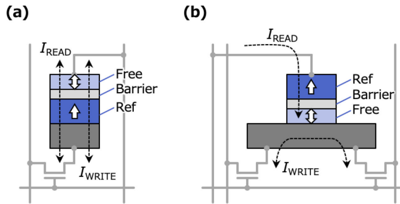
Figure 10. Typical cell structure of STT-MRAM (a) and SOT-MRAM (b). Exemplary magnetization directions are indicated by white arrows and write I_{\text{WRITE}} and read I_{\text{READ}} current paths are indicated by broken arrows.
