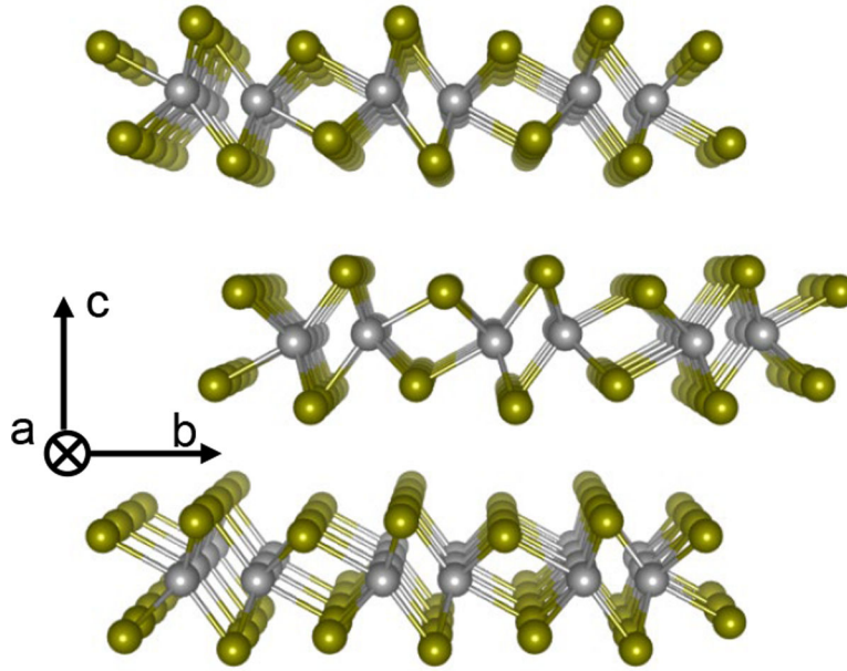
Figure 9. Crystal structure of 1T_d -WTe 2 , where the grey and sycamore colored atoms represent W and Te, respectively. Note that there is only one mirror plane – bc plane.
