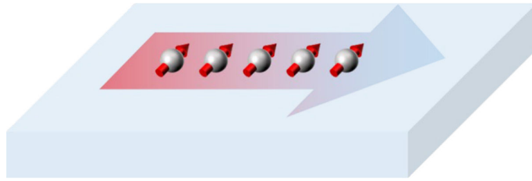
Figure 5. Schematic of thermal gradient-induced spin current.
