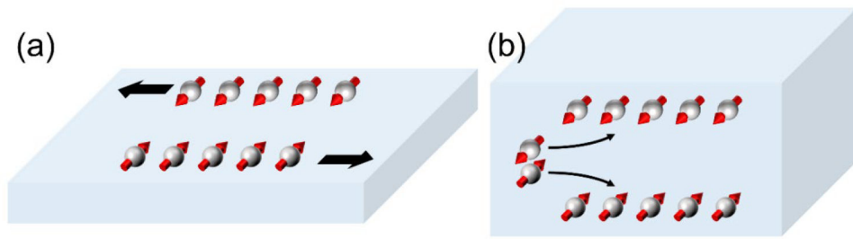
Figure 3. Schematics of (a) Rashba-Edelstein effect and (b) spin Hall effect
