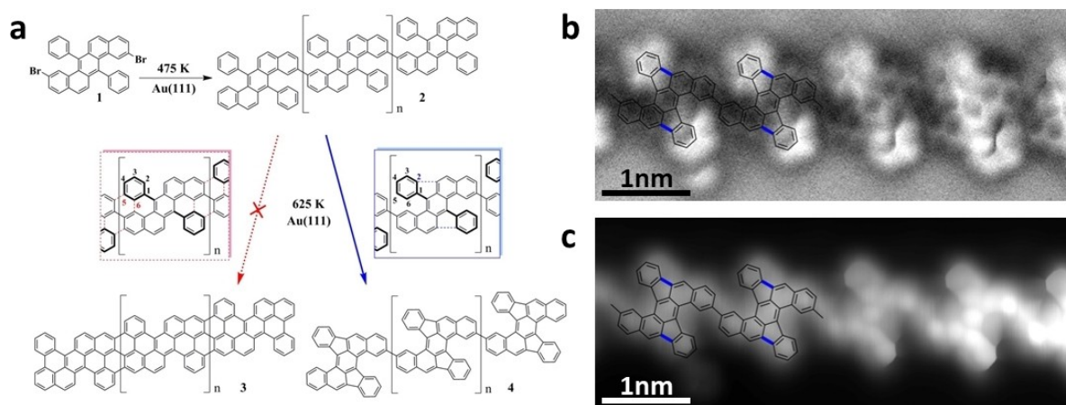
Figure 2. a) Schematics of the polymerization of 2,9-dibromo-7,14-diphenylbenzo[ k ]tetraphene ( 1 ) into polymer 2 . Following the formation of polymer 2 , two CDH pathways involving the phenyl substituents are possible: they may either form two six-membered rings resulting in a cove-edged graphene nanoribbon ( 3 , red path), or a five-membered ring yielding a new type of polymer consisting of dibenzo[ a,m ]rubicene repeat units ( 4 , blue path). The nc-AFM frequency-shift image (b) and simultaneously recorded current image (c) clearly reveal the formation of five-membered rings, and thus identify 4 as the experimentally obtained reaction product ( V = -5 mV).
