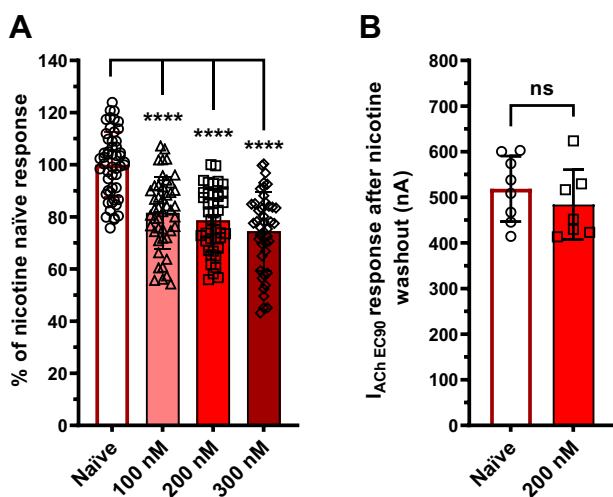
Figure 3. Nicotine driven \alpha 7 nAChR desensitization. A, nicotine desensitized \alpha 7 nAChRs in a concentration-dependent manner (right) ( N = 4 , n = 42-52 ) (One-Way ANOVA with Dunnett's posthoc analysis, F(3,12) = 32.09 , ****p < 0.0001 ). Data was collected at the second ACh application after full-agonist response has been demonstrated (96). B, upon recovery, nicotine pretreated \alpha 7 nAChRs showed no increase in macroscopic ACh responses (left) ( N = 3 , n = 7-9 ) (Welch's two-tailed t test t(4) = 0.33 , {}^{ns}P = 0.757 ). All points are the mean \pm SD. ACh, acetylcholine; nAChR, nicotinic acetylcholine receptor.
