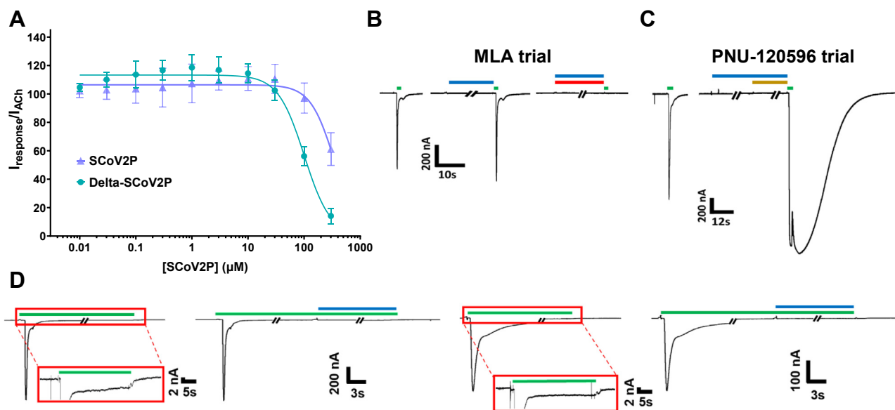
Figure 5. \alpha 7 nAChR current responses to pharmacological ligands reveals SCoV2P mechanisms of action. A, normalized delta SCoV2P-induced alterations in ACh-induced responses as a percentage of control response. Previously presented SCoV2P data is included to facilitate comparison. The single point mutation found in the neurotoxin-like region caused a significant change in inhibition potency (One-Way ANOVA with Tukey's posthoc analysis F(4, 14) = 10.04 , ***p = 0.0002 ). B, MLA (red) blocks SCoV2P (blue) and ACh (green)-induced currents. C, SCoV2P coapplied with PNU-120596 (gold) does not induce a current nor does SCoV2P block PNU-120596 modulation of ACh-mediated currents. D, SCoV2P is not capable of directly reactivating desensitized receptors but instead facilitates receptors to recover from being desensitized (i.e., return to the closed state). Experiments were conducted at ACh EC_{100} (top) and at EC_{20} (bottom) concentrations. The red box enlargement is showing that receptors are in steady state after a 30 s application of ACh. All experiments were performed on at least two individual animals and at least three oocytes. ACh, acetylcholine; MLA, methyllycaconitine; nAChR, nicotinic acetylcholine receptor; SCoV2P, SARS-CoV-2 glycoprotein peptide.
