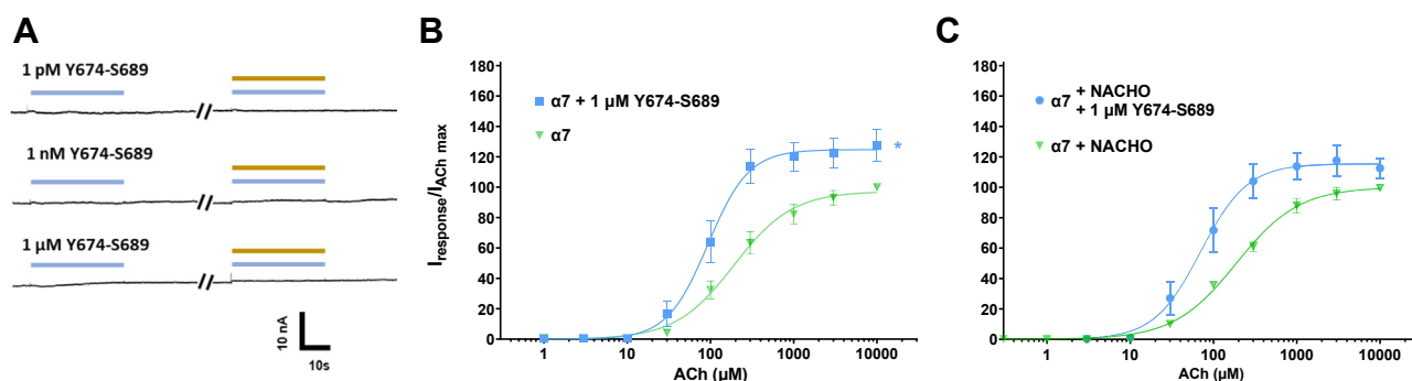
Figure 6. Y674-S689 positively modulates \alpha 7 nAChRs expressed in absence and with the chaperone protein NACHO. A, raw recordings showing currents in presence of 1 \mu M Y674-S689 (light blue) and 10 \mu M PNU-120596 (gold) show that no \alpha 7 nAChR activation occurred. Each set of traces were collected from unique oocytes ( N = 3 , n = 3-5 ). B, one \mu M Y674-S689 significantly enhanced ACh potency (One-Way ANOVA with Tukey's posthoc analysis F(3, 9) = 69.12 , ****p < 0.0001 ) and efficacy (One-Way ANOVA with Tukey's posthoc analysis F(3, 9) = 6.682 , *p = 0.0163 ). C, \alpha 7 nAChRs co-expressed with NACHO showed similar and 1 \mu M Y674-S689 responses as \alpha 7 nAChRs expressed alone, with 1 \mu M Y674-S689 significantly enhancing ACh potency (One-Way ANOVA with Tukey's posthoc analysis F(3, 9) = 69.12 , ****p < 0.0001 ). All points are the mean \pm SD. Data values are reported in Tables S4. ACh, acetylcholine; nAChR, nicotinic acetylcholine receptor.
