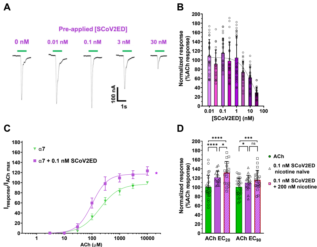
Figure 9. SCoV2ED potentiates and inhibits ACh \alpha 7 nAChRs with nanomolar potency. A , \alpha 7 nAChR ACh-evoked currents were measured by TEVC using cRNA injected Xenopus laevis oocytes. SCoV2ED (0.01–30 nM) was applied for 5 min prior to ACh stimulation. Green drug application bars indicate the time 1300 \mu M ACh was applied. B , increasing concentrations of SCoV2ED inhibited ACh-induced responses. Data were normalized to the control response (40% PBS). Data are the mean \pm SD (N = 5, n = 25–44). Nonlinear regression curve fit to SCoV2ED data with an IC 50 of 11 \pm 6 nM. C , 0.1 nM SCoV2ED enhances ACh potency from 192 \mu M [CI 174, 212] to 102 \mu M [CI 93, 111] (student's unpaired t test, t = 4.625, df = 6, **p = 0.0036). ACh maximal responses were also significantly enhanced (123 \pm 9%) (student's unpaired t test t = 3.207, df = 5, *p = 0.0238) when compared to \alpha 7 nAChRs that were not exposed to SCoV2ED (N = 3–5, n = 9–14). D , at the ACh EC 20 and EC 90 , 0.1 nM SCoV2ED (solid purple bar) significantly potentiated the ACh-mediated response (solid green bar). With 200 nM nicotine preincubation (hashed purple bar), 0.1 nM SCoV2ED significantly potentiated the ACh-induced control response (40% PBS) and in the case of the EC 20 data greater than the 0.1 nM SCoV2ED enhanced currents (N = 3, n = 16–21) (One-way ANOVA with Tukey's multiple comparison test F(5,12) = 49.85 , ^{13}P = 0.2715 , *p < 0.05 , ***p = 0.0007 , ****p < 0.0001 ). Data are the mean \pm SD. ACh, acetylcholine; nAChR, nicotinic acetylcholine receptor; SCoV2ED, SARS-CoV-2 ectodomain; TEVC, two-electrode voltage clamp.
