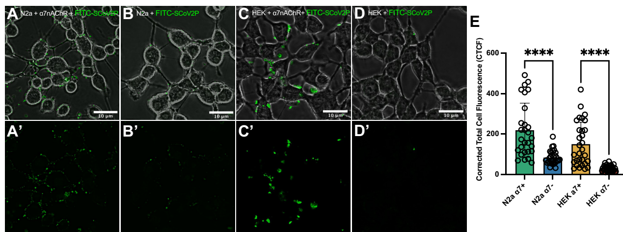
Figure 7. SCov2P preferentially interacts with cells expressing \alpha 7 nAChRs. Live-cell confocal images of 50 \mu M FITC-SCov2P treated (A) \alpha 7 nAChR-transfected N2a, (B) nontransfected N2a, (C) \alpha 7 nAChR-transfected HEK293, and (D) \alpha 7 -null HEK293 cells. (A'–D') Same as (A–D) without displaying the phase channel. E, CTCF of 24 h incubation of FITC-SCov2P with \alpha 7 nAChR-transfected N2a and HEK293 cells, as well as nontransfected N2a and HEK293 cells (number of analyzed cells (n) = 30, student's unpaired t test t = 5.350, df = 56 (N2a); t = 5.983, df = 58 (HEK293), **** p < 0.0001). All points are mean \pm SD. CTCF, corrected total cell fluorescence; HEK293, human embryonic kidney 293; nAChR, nicotinic acetylcholine receptor; SCov2P, SARS-CoV-2 glycoprotein peptide.
