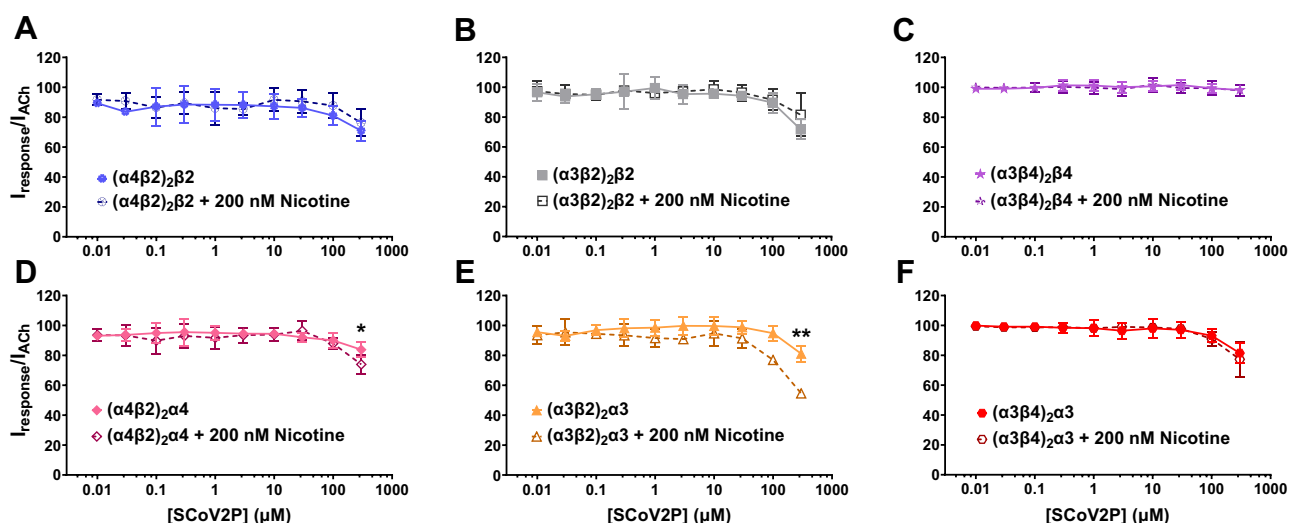
Figure 1. SCoV2P minimally inhibits ACh-invoked heteromeric nAChR responses. Data are grouped by isoform and normalized to ACh-induced responses without SCoV2P application. Significant changes are noted with * and were determined for 300 \mu\text{M} SCoV2P difference between nicotine naïve and 200 nM nicotine preincubation responses (Welch's two-tailed t test: (\alpha 4\beta 2)_2\alpha 4 t(7.2) = 2.57 , *p = 0.036 ; (\alpha 4\beta 2)_2\alpha 3 t(6.8) = 4.46 , **p = 0.0032 ). A–C, high agonist sensitivity nAChRs were minimally inhibited with SCoV2P and nicotine treatment had no effect. D–F, low agonist sensitivity nAChRs experienced an increase in SCoV2P-induced inhibition with nicotine presence. Points are the mean \pm SD ( N = 3 , n = 3 –5). ACh, acetylcholine; nAChR, nicotinic acetylcholine receptor; SCoV2P, SARS-CoV-2 glycoprotein peptide.
