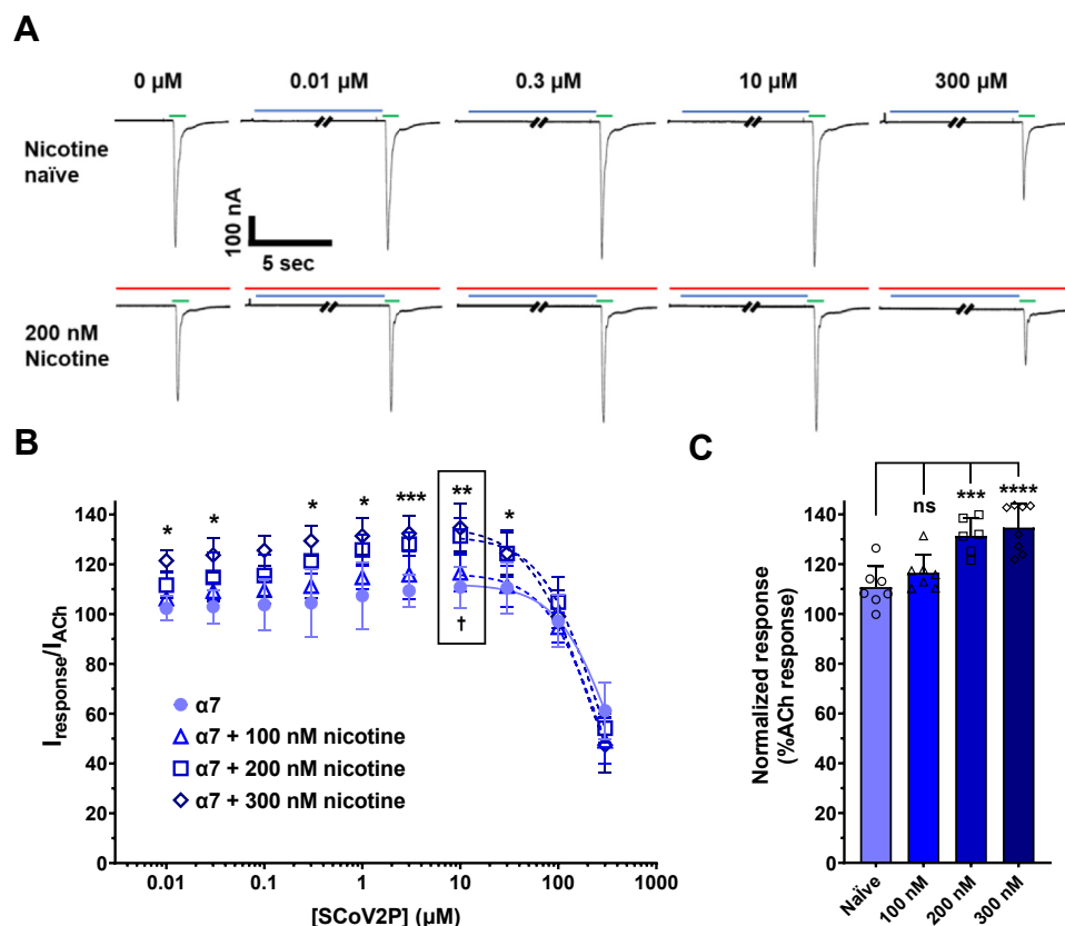
Figure 2. SCoV2P modulation of homomeric \alpha 7 nAChRs. A, current recordings generated using cRNA injected Xenopus laevis oocytes displaying alterations in ACh-induced currents after preapplication of increasing SCoV2P concentrations (0.01–300 \mu M). Thirty seconds SCoV2P preapplications are shown in blue, while 1 s ACh stimulations are displayed in green (coloring scheme is applicable to all displayed recordings). B, normalized SCoV2P-induced alterations in ACh-induced responses as a percentage of control response. SCoV2P significantly potentiates (Two-tailed one sample t test t(4) = 3.41 , ^{\dagger}p = 0.0271 ) and inhibits ACh-induced currents. Nicotine 200 and 300 nM pretreatments augment the SCoV2P effect. Significant changes are noted with * to indicate differences between nicotine naïve and 200 nM nicotine treatment group ( N = 3-5 , n = 7-9 ) (Welch's two-tailed t test t(4.3-7.9) = 2.28-5.77 , *p < 0.05 , **p = 0.0014 , ***p = 0.0005 ). The box identifies maximal potentiation induced using 10 \mu M SCoV2P. All points are the mean \pm SD. C, ten \mu M SCoV2P significantly potentiates ACh currents, which are further enhanced with increasing nicotine concentrations (One-Way ANOVA with Tukey's posthoc analysis F(3, 24) = 14.00 , ***p = 0.0005 , ****p < 0.0001 ). ACh, acetylcholine; nAChR, nicotinic acetylcholine receptor; SCoV2P, SARS-CoV-2 glycoprotein peptide.
