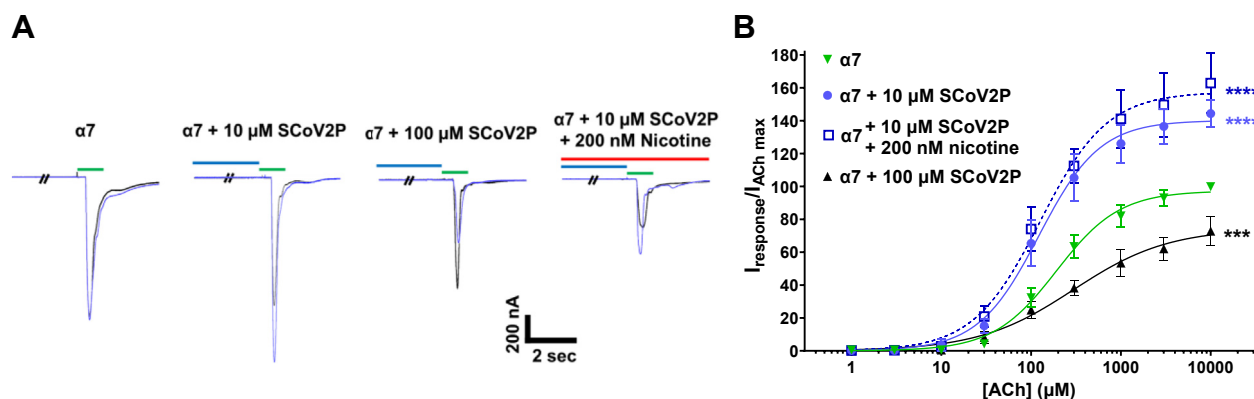
Figure 4. SCoV2P allosteric modulation of \alpha 7 nAChRs. A, raw recordings showing ACh maximal (10 mM) currents in the absence (black) and presence (blue) of 10 or 100 \mu\text{M} SCoV2P and preincubated with 200 nM nicotine (10 \mu\text{M} SCoV2P). Each set of traces were collected from unique oocytes. B, ten \mu\text{M} SCoV2P enhances ACh potency, in addition to enhancing ACh-induced responses significantly. A higher SCoV2P concentration (100 \mu\text{M} ) reduced ACh potency and efficacy (One-Way ANOVA with Tukey's posthoc analysis F(3,13) = 144.8 , ***p = 0.0003 , ****p < 0.0001 ). All points are the mean \pm SD. Data values are reported in Tables S2 and S3. ACh, acetylcholine; nAChR, nicotinic acetylcholine receptor; SCoV2P, SARS-CoV-2 glycoprotein peptide.
