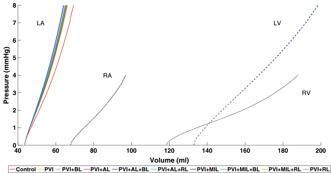
FIGURE 4. End-diastolic pressure–volume relationship (EDPVR) for the left atrium (LA), right atrium (RA), left ventricle (LV) and right ventricle (RV) for all simulations.
