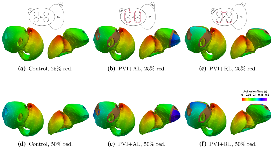
FIGURE 11. Activation time map and isochrones for the Control (a + d), the PVI + AL (b + e), and the PVI + RL (c + f) cases with a 25 and 50% reduction in conductivity.
