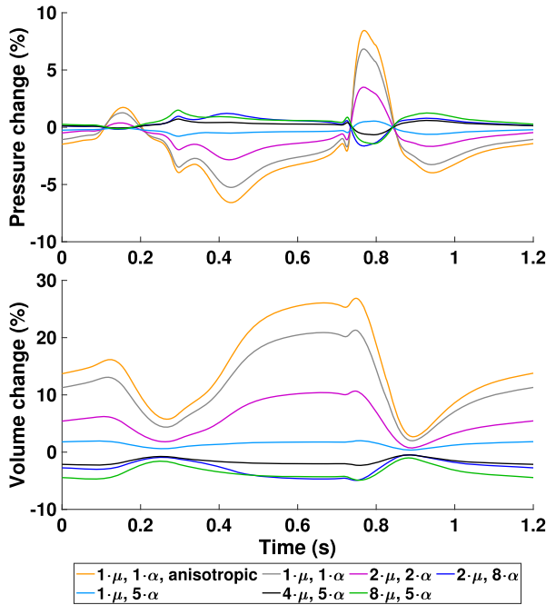
FIGURE 10. Simulation results of the case PVI + AL + BL for varying scar stiffness. The change in pressure and volume of the left atrium is relative to a PVI + AL + BL reference simulation with 2 \cdot \mu and 5 \cdot \alpha and normalized by their peak-to-peak values.
