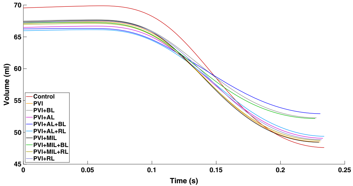
FIGURE 5. Blood volume traces during left atrial systole. Atrial systole lasts from the externally applied stimulation of the sinus node to the time of maximal contraction of the left atrium.
