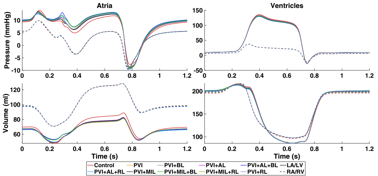
FIGURE 8. Atrial (left column) and ventricular (right column) pressure (top row) and volume (bottom row) courses during one heart cycle. Different colors denote the simulation results of the healthy control case and all simulations including scars. Left atrium and ventricle are shown with solid lines while right atrium and ventricle are shown with dashed lines.
