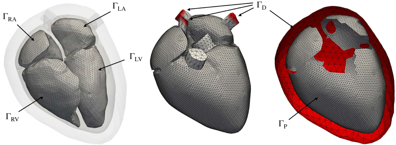
FIGURE 1. Surfaces on which boundary conditions are applied: the endocardial surfaces \Gamma_n = \Gamma_{LV} \cup \Gamma_{RV} \cup \Gamma_{LA} \cup \Gamma_{RA} are used for the pressure boundary condition; \Gamma_D is used as a zero displacement Dirichlet boundary; and \Gamma_P is used for the frictionless sliding contact problem. Note that the Dirichlet boundary in the right figure is clipped for visualization reasons.
