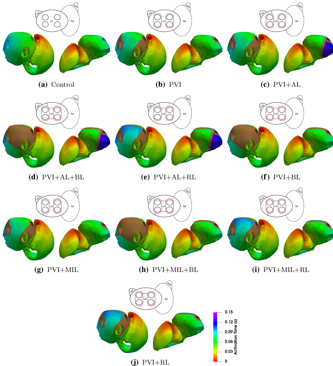
FIGURE 3. Activation maps and isochrones of the depolarization wave in sinus rhythm. A brown color denotes inactive tissue. The pictogram of the atria at the top of each model indicates the applied ablation lesions (red lines).
