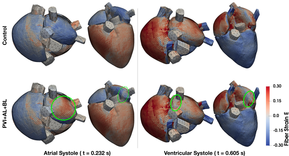
FIGURE 7. Green Lagrange strain E_{fr} in fiber direction of the Control and PVI + AL + BL case is shown in superior and anterior view during atrial and ventricular systole, respectively. Green circles mark the areas of increased/decreased strain referred to in the text.
