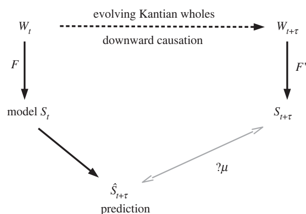
Figure 1. A schematic and abstract view of the main elements and relations involved in our argument. W_t denotes the ‘world’ at time t ; after an interval \tau the world changes. Biological evolution with the emergence of new Darwinian preadaptations and new relevant variables occurs. Organisms are Kantian wholes where the parts exist in the universe for and by means of the whole. Natural selection is downward causation . The explanatory arrows point upward . What comes to exist cannot be deduced from below. Reductionism fails. Selection acts on the Kantian whole and propagates its parts as they evolve new adaptations to better sustain the Kantian whole. We can use no mathematics based on set theory to deduce these new adaptive features. Thus there is no mathematical mapping based on set theory and perhaps more broadly from the biological world at time t to the biological world at t + \tau . Therefore, the hope for a mapping \mu that is a prediction from a model of the world at time t + \tau to the actual world at t + \tau does not exist. We can neither deduce the evolution of the biosphere nor estimate the errors in our predictions.
