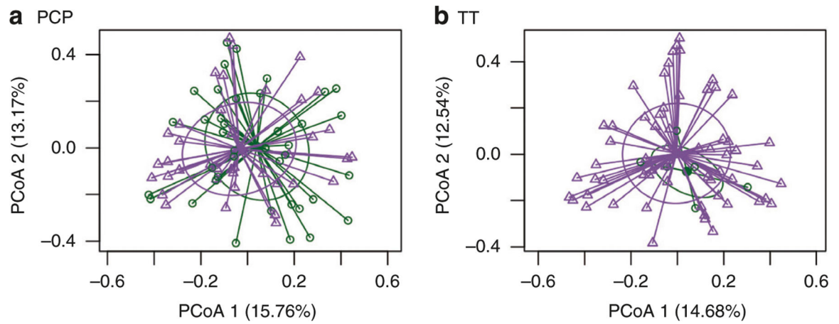
Fig. 1. PCoA plots of bacterial 16S V4-V5 rRNA sequencing Bray-Curtis dissimilarity for PCP and TT.
