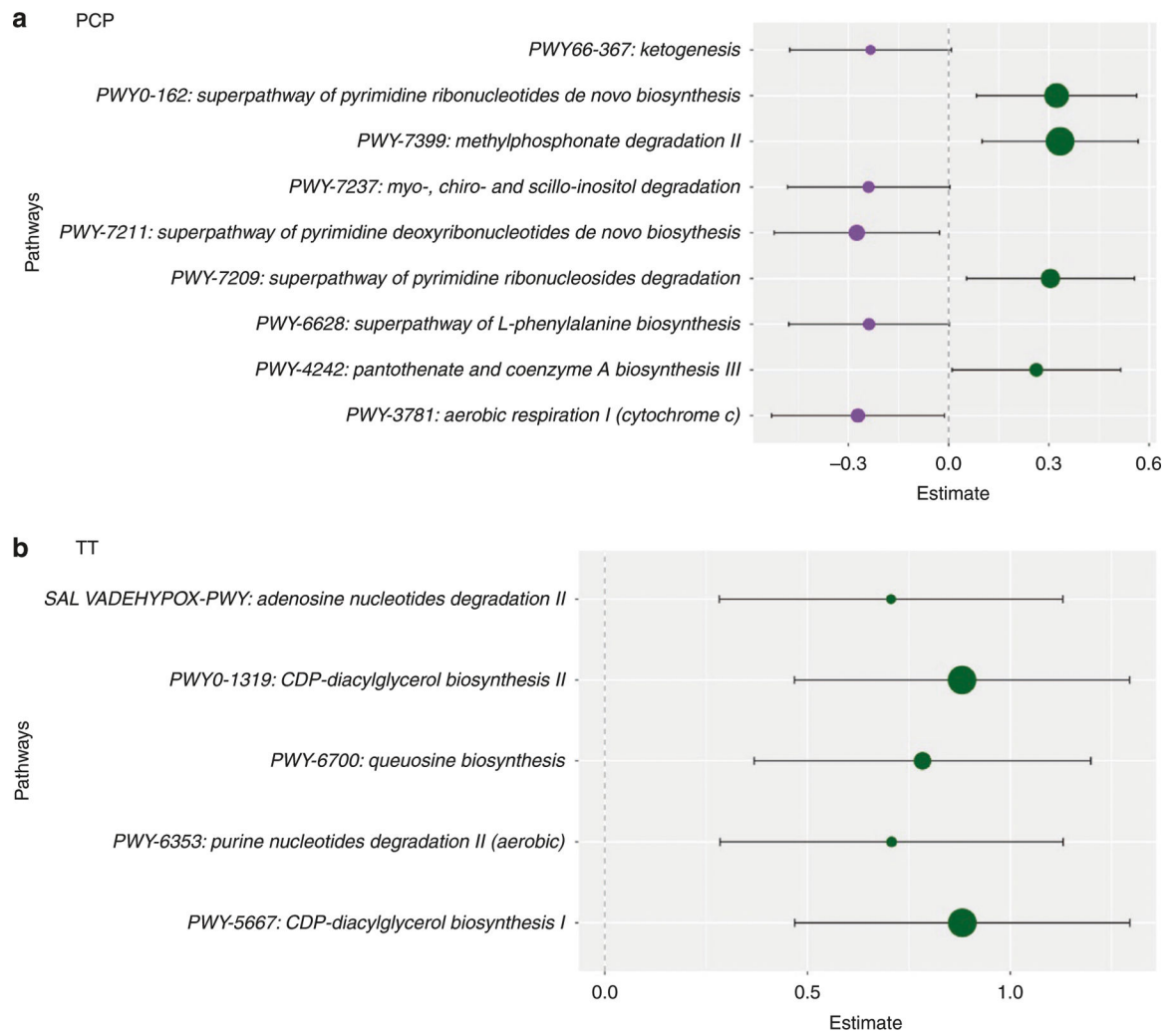
Fig. 3. Associations between elastic-net and metabolic pathways and vaccine response. Dots indicate effect size, and horizontal bands indicate 95% CI. Green dots represent positive association, while purple dots represent negative association. Size of dots vary by p value: larger dot indicates smaller p value. Only pathways selected by elastic net and FDR correction shown here. a Metabolic pathways associated with PCP response. b Metabolic pathways associated with TT response.
