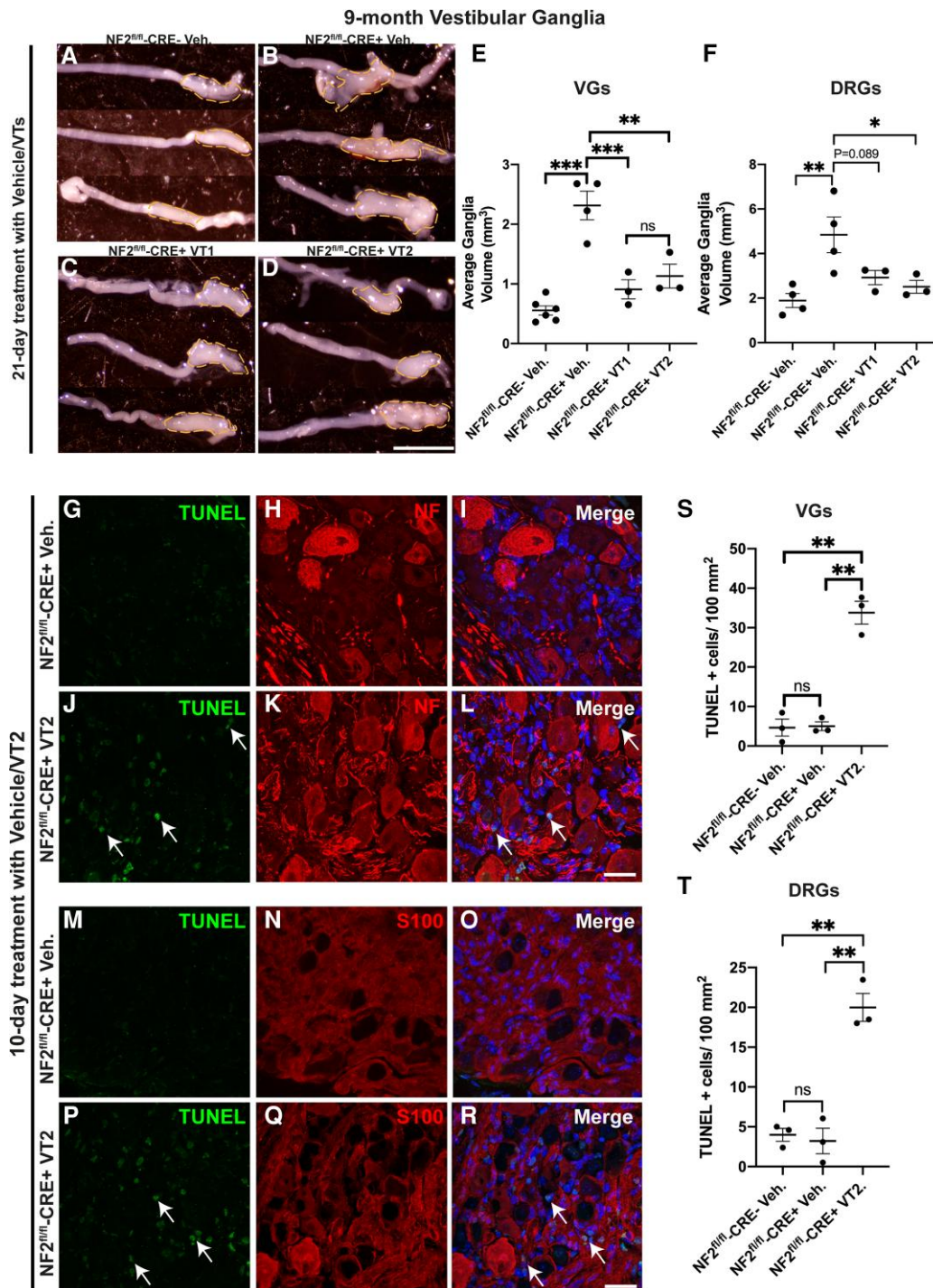
Figure 3 Treatment of mice with VT auto-palmitoylation inhibitors significantly increases apoptosis and reduces tumour volumes in VG and DRG in 9-month-old NF2^{fl/fl} - CRE+ ( NF2^{fl/fl} - CRE+ ) mice. NF2^{fl/fl} - CRE- ( NF2^{fl/fl} - CRE- ) and NF2^{fl/fl} - CRE+ animals were treated with vehicle (Veh), 10 mg/kg/day VT1 or 30 mg/kg/day VT2 by oral gavage for 10 or 21 consecutive days. (A–D) Representative brightfield micrographs of three different unilateral VG from: NF2^{fl/fl} - CRE- Veh-treated mice (A), NF2^{fl/fl} - CRE+ Veh-treated mice (B), NF2^{fl/fl} - CRE+ VT1-treated mice (C) and NF2^{fl/fl} - CRE+ VT2-treated mice (D), all mice were treated for 21 consecutive days. Scale bar = 20 \mu m. (E) Quantification of average bilateral VG volume in A–D, for NF2^{fl/fl} - CRE- Veh-treated mice ( n = 6 ganglia, n = 3 mice), NF2^{fl/fl} - CRE+ Veh-treated mice ( n = 4 ganglia, n = 3 mice), NF2^{fl/fl} - CRE+ VT1-treated mice ( n = 3 ganglia, n = 3 mice) and NF2^{fl/fl} - CRE+ VT2-treated mice ( n = 3 ganglia, n = 3 mice). (F) Quantification of average bilateral lumbar 4 DRG volume, for NF2^{fl/fl} - CRE- and NF2^{fl/fl} - CRE+ Veh-treated mice ( n = 8 ganglia, n = 3 mice), for NF2^{fl/fl} - CRE+ VT1- and NF2^{fl/fl} - CRE+ VT2-treated mice ( n = 3 ganglia, n = 3 mice). (G–R) Representative immunofluorescence of n = 3 different VGs with in situ apoptosis detected by terminal deoxynucleotidyl transferase dUTP nick-end labelling (TUNEL) assay, following oral gavage with either vehicle or 30 mg/kg/day VT2 for 10 days. TUNEL + nuclei (arrows; J, L, P and R) were significantly increased in NF2^{fl/fl} - CRE+ VT2-treated mice compared to NF2^{fl/fl} - CRE+ Veh-treated mice. Neurofilament (NF; H and K) counterstain (merged with Hoechst counterstain (I and L)) reveals increased apoptosis in cells surrounding neuronal cell bodies of the VG in NF2^{fl/fl} - CRE+ VT2-treated mice. S100 counterstain (N and Q merged with Hoechst counterstain (O and R)) reveals apoptosis is increased in S100+ schwannoma cells of NF2^{fl/fl} - CRE+ VT2-treated mice. Scale bars = 20 \mu m. (S and T) Quantification of TUNEL + cells/100 mm 2 in VG (S) and DRG (T). In E and F, data presented as mean \pm SEM using one-way ANOVA with Tukey’s multiple comparisons tests. In S and T, data presented as mean \pm SEM using Brown–Forsythe and Welch ANOVA with Dunnett’s T3 multiple comparisons test. ** P < 0.01 ; *** P < 0.001 ; ns = non-significant.
