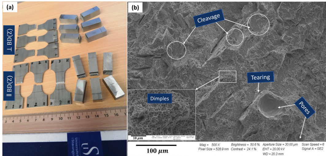
Fig. 21. (a) The ruptured mechanical test samples. (b) Fracture surface of the Charpy specimen.
