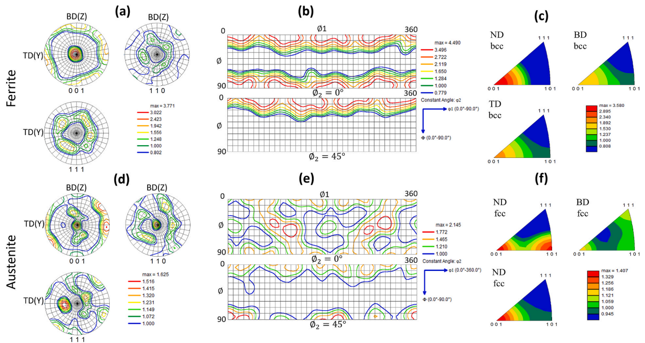
Fig. 15. (a, d) Pole figures, (b, e) ODF sections \phi_2 = 0^\circ, 45^\circ and (c, f) IPFs of \alpha and \gamma in layer L2.
