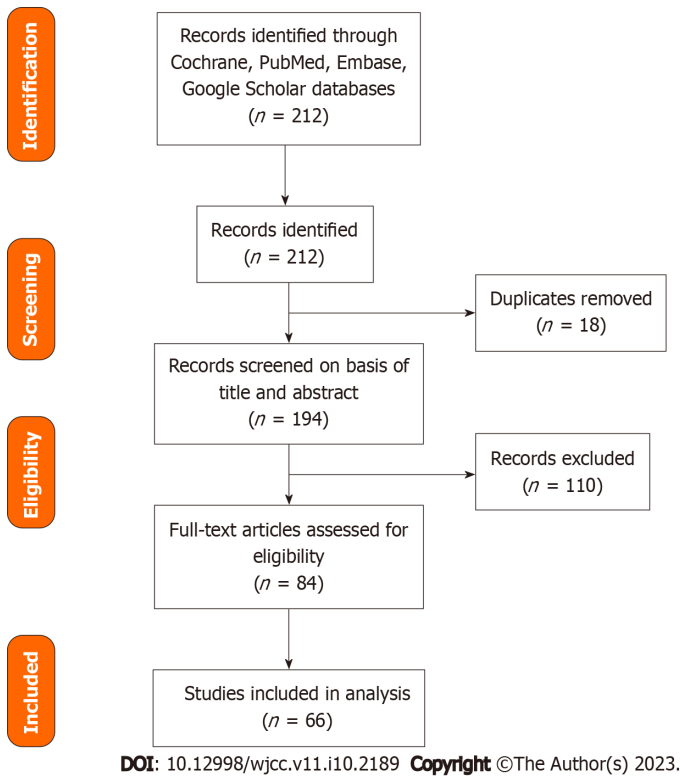
Figure 1 Prisma flowchart.
