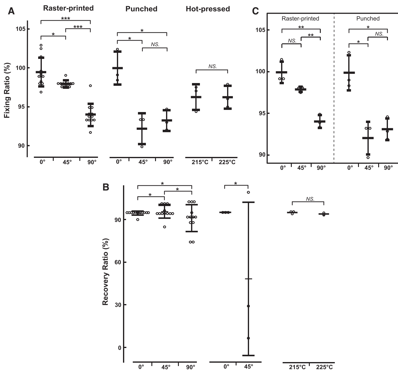
FIG. 4. (A) Fiber orientation affects fixing ratio in both raster-printed and punched samples. Crossbars on standard deviations show group means ( *p < 0.05 ; ***p < 0.001 , Tukey's HSD post hoc ). No significant effects were found for the hot-pressed control groups. (B) Fiber orientation significantly affects the variance of recovery ratio of both raster-printed and punched samples. Crossbars on standard deviations show group means ( *p < 0.050 by Bartlett's test for raster-printed samples and F-test for punched samples). No significant effects were found for the hot-pressed control groups. (C) For only the subset of samples from (A) printed at 225°C with a multiplier of 1.0, interactions between fiber orientation and fabrication method have a significant effect on fixing ratio. Crossbars on standard deviations show group means ( *p < 0.05 ; ***p < 0.005 ; NS p > 0.05 , Tukey's HSD post hoc ). For the polynomial regressions (raster-printed sample fixing and recovery ratios) and piecewise linear regression (punched sample fixing ratio), \theta is in units of degrees. HSD, Tukey's honestly significant difference test; NS, no significant difference.
