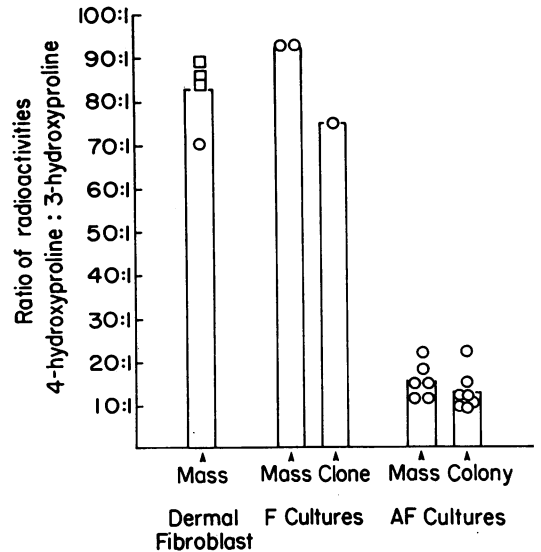
Fig. 4 The proportions of radioactive 4- and 3-hydroxyproline in collagen prepared from the culture medium of various types of cultures. Each point is for a different culture, most of which are also represented in Fig. 3. □ denotes non-fetal cultures. Tops of bars represent mean values.
