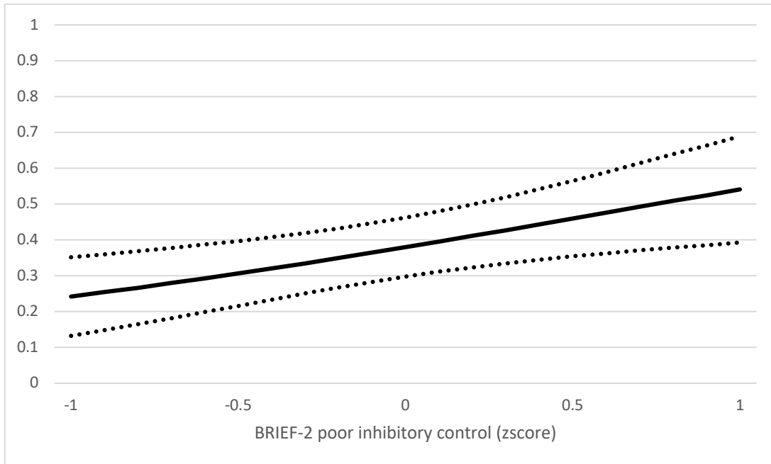
Figure 2. Probability of Marijuana Initiation by BRIEF Inhibitory Control
