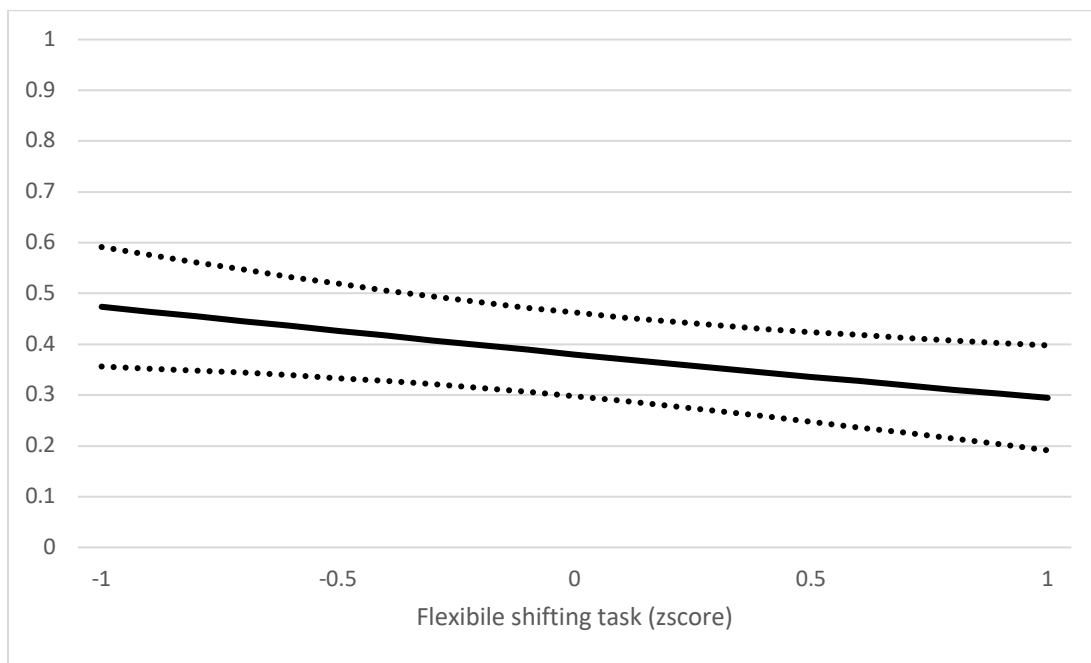
Figure 1. Probability of Marijuana Initiation by Flexible Shifting Task
