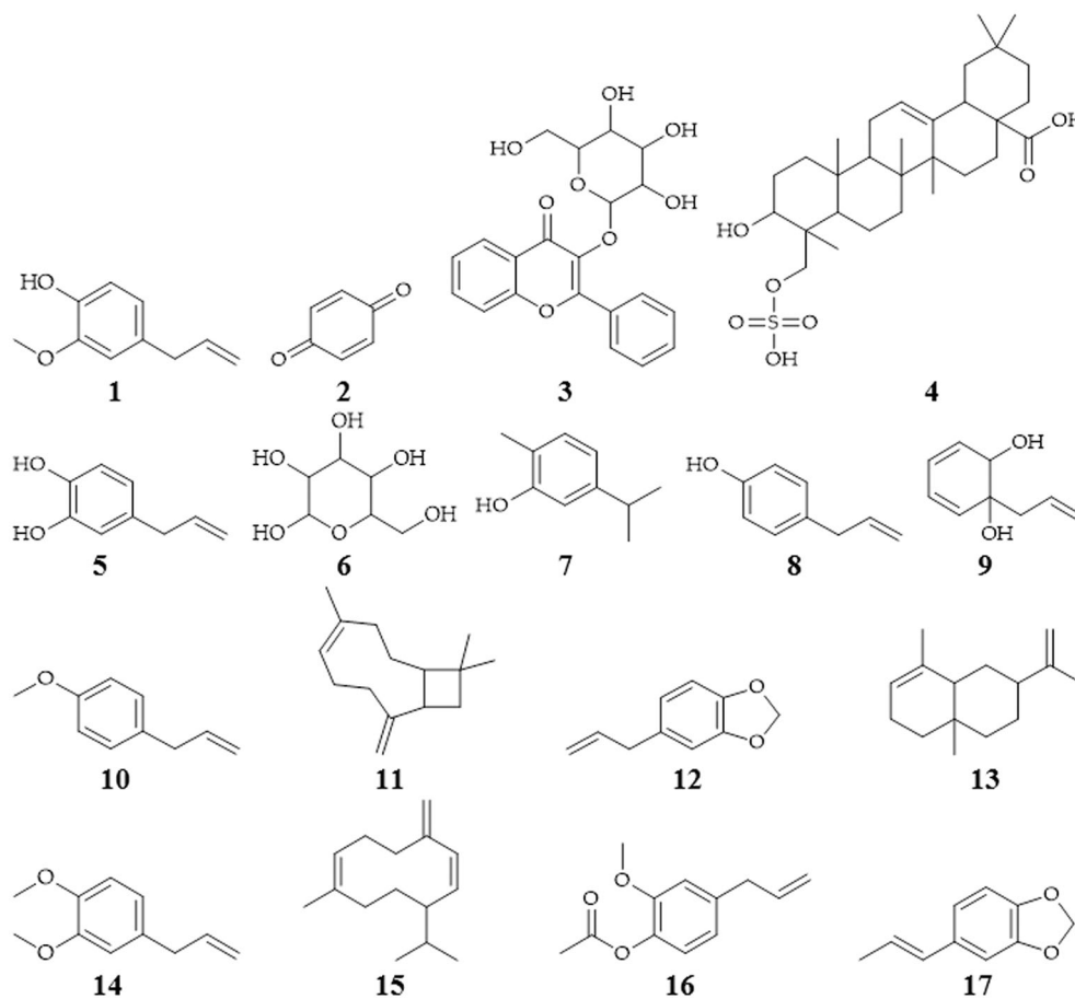
Figure 2. Chemical structures of P. crocatum (Saputra et al. 2016; Fatmawaty et al. 2019; Lister et al. 2020).
