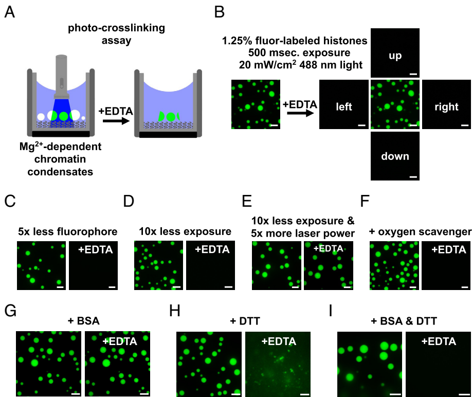
Fig. 5. DTT and BSA mitigate photocrosslinking during fluorescence microscopy. (A) Diagram depicting an assay to detect photocrosslinking of intrinsic chromatin condensates. (Left) Magnesium-dependent intrinsic chromatin condensates are exposed to fluorescent light prior to the addition of superstoichiometric quantities of EDTA. (Right) Photocrosslinked condensates fail to dissipate following chelation of magnesium. (B) Confocal fluorescence microscopy images of intrinsic chromatin condensates composed of nucleosomal arrays where 1 in 80 histone molecules are labeled with AlexaFluor 488. Images are following exposure to fluorescent light and both before (Left) and after (Right) the addition of EDTA. Confocal fluorescence microscopy images of intrinsic chromatin condensates imaged, as in Fig. 5B, with (C) less fluorophore, (D) less exposure, (E) more laser power with less exposure, or (F) the inclusion of oxygen scavenging components. Confocal fluorescence microscopy images of intrinsic chromatin condensates formed in the presence of (G) BSA, (H) DTT, or (I) BSA and DTT and imaged as described in Fig. 5B. Fluorescent microscopy images before and after the addition of EDTA were processed separately. All experiments were performed using nucleosome arrays with 25 base pair internucleosome repeat length. Scale bars, in white, are 10 \mu\text{m} .
