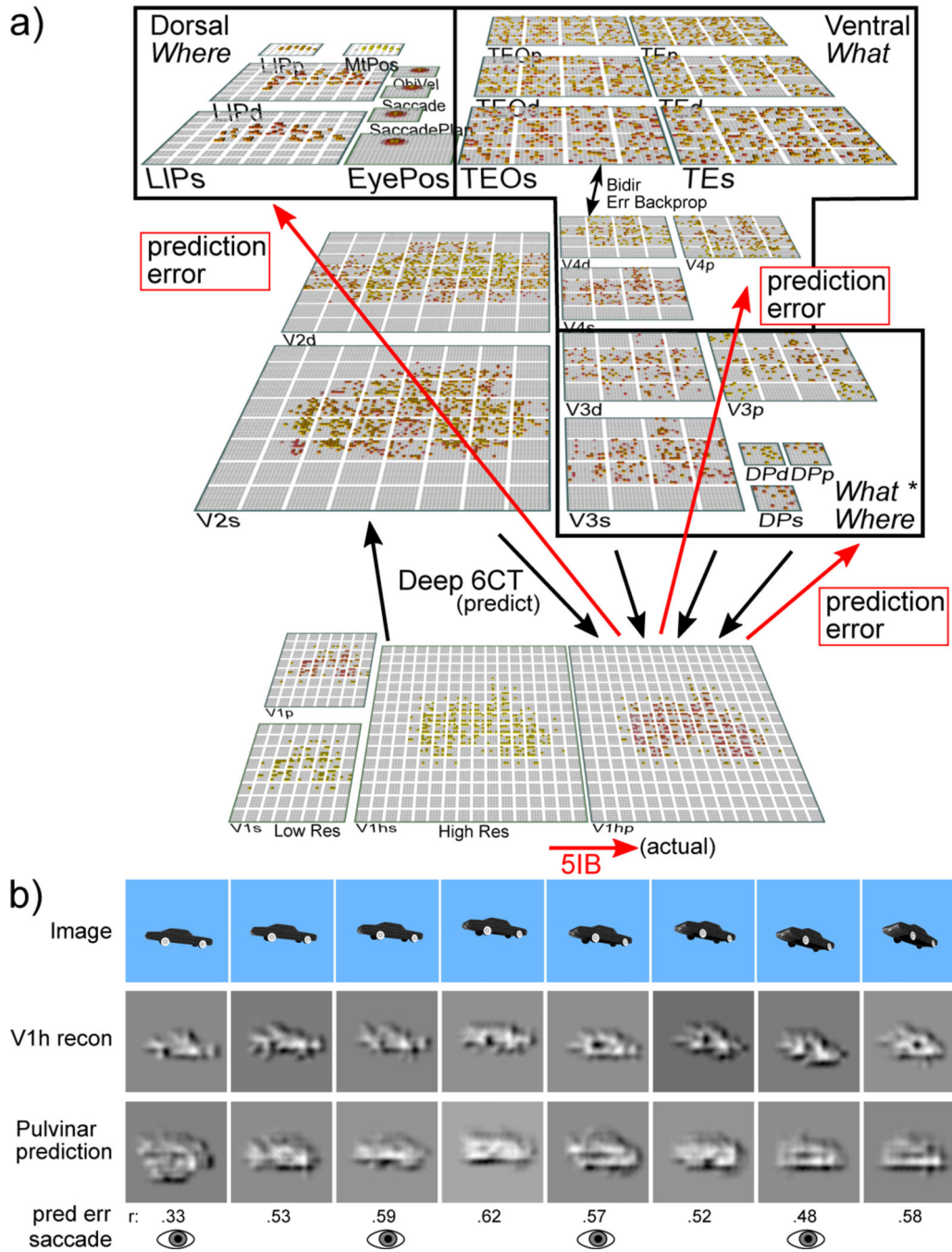
Figure 5: a) The What-Where-Integration , WWI deep predictive learning model. The dorsal Where pathway learns first, using easily-abstracted spatial blobs , to predict object location based on prior motion, visual motion, and saccade efferent copy signals. This drives strong top-down inputs to lower areas with accurate spatial predictions, leaving the residual error concentrated on What and What * Where integration. The V3 and DP (dorsal prelunate) constitute the What * Where integration pathway, binding features and locations. V4, TEO, and TE are the What pathway, learning abstracted object category representations, which
