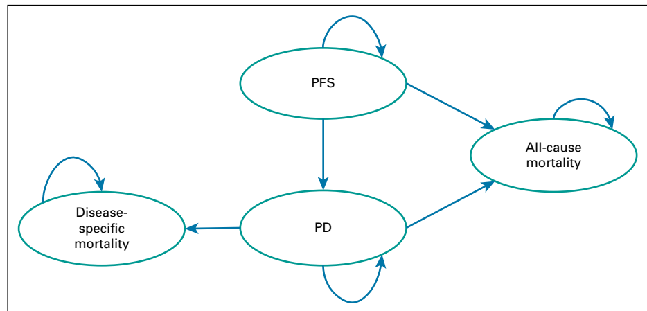
FIG 1. Schematic diagram for the Markov state transition model. PD, progressive disease; PFS, progression-free state.
