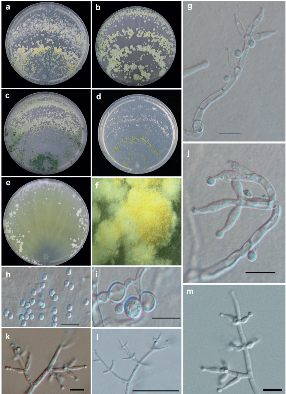
Figure 4. Cultures and anamorph of T. paradensissimum strain T31823 a–d cultures on different media at 25 °C with a 12 h light and 12 h darkness cycle after 7 d ( a on PDA b on MEA c on CMD d on SNA) e culture on PDA at 35 °C with darkness after 7 d f conidiation pustules on PDA after 7 d g, j–m conidiophores and phialides ( g, j on CMD 3 d k–m on SNA 3 d) h conidia i chlamydo-spores. Scale bars: 10 µm ( g–m ).
