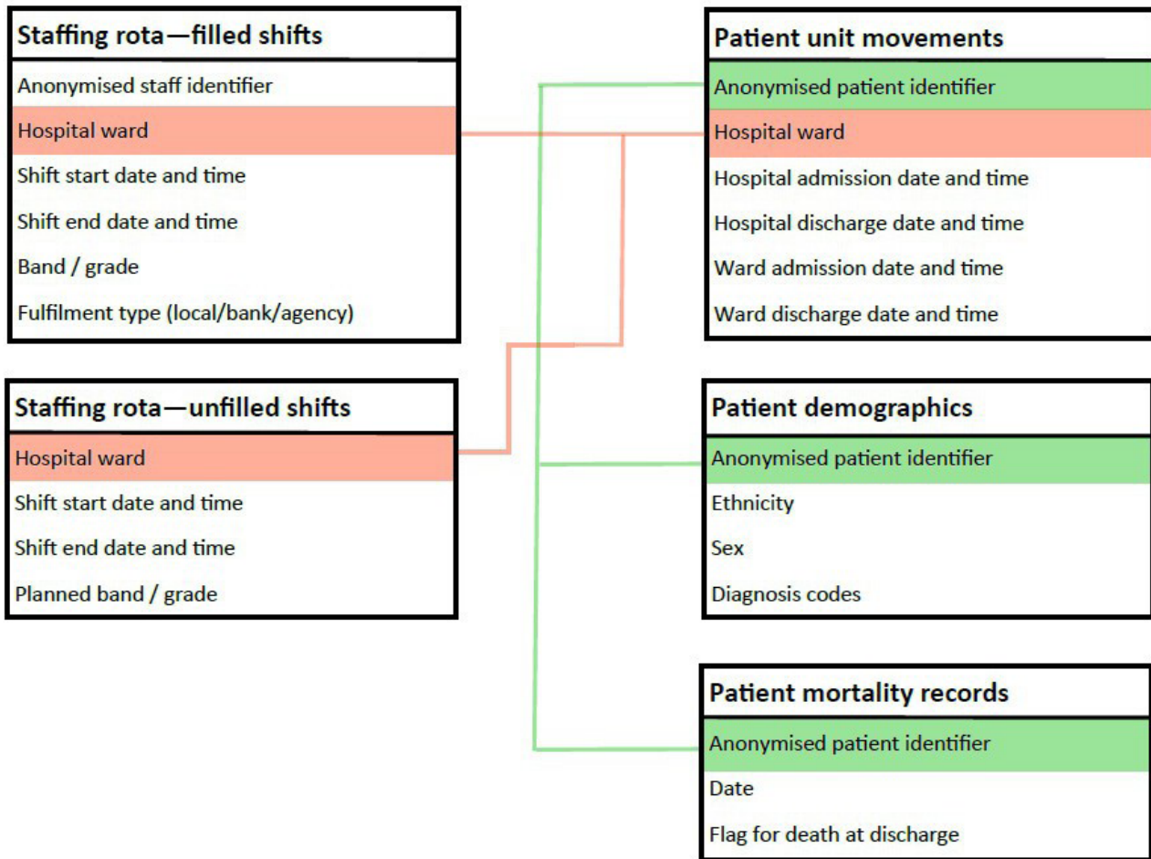
Figure 1 Data structure.
