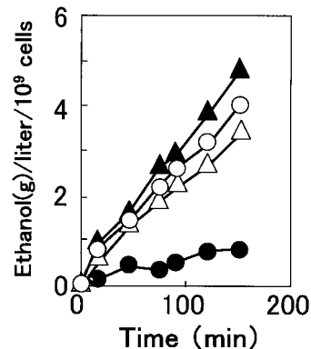
FIG. 1. Ethanol production by permeabilized (open symbols) and intact (solid symbols) cells of the parent strain YHK142 (triangles) and the disruptant strain YHK1144 (circles) at 10°C. Cells were suspended in a buffer containing 5 mM MgCl 2 , 2 mM ATP, 1 mM NAD + , 30 mM P i , 1 mM arsenate, and 150 mM MES (pH 6.9). Ethanol fermentation was initiated by addition of glucose (final concentration, 2%).
