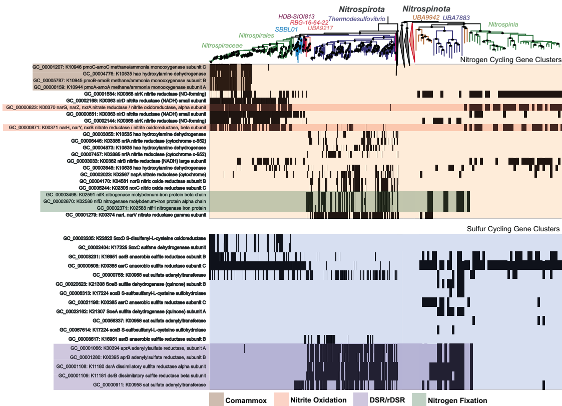
Fig. 6 Presence/absence patterns of gene clusters with annotations involved in the Nitrogen cycling (KO Ids included in KEGG Map M00910) and Sulfur cycling (KO Ids included in KEGG Map M00920) in Nitrospirota and Nitrospinota . The rows are ordered by hierarchical clustering of presence/absence patterns in Nitrospirota using Ward's Linkage. Functional differences and similarities between the two phyla can be noted. The shaded boxes denote functions of interest that are discussed in the text.
