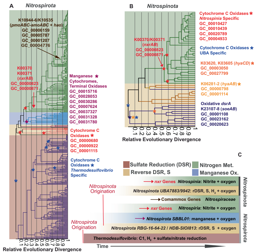
Fig. 8 Proposed scheme of metabolic progression throughout the histories of Nitrospirota and Nitrospinota. A The phylogeny of Nitrospirota scaled with Relative Evolutionary Divergence (RED) (x axis), as used to denote particular taxonomic ranks by GTDB. The branches are colored in the same fashion as Fig. 1. The taxonomic groups are colored by boxes denoting the main metabolisms of those groups as defined in panel (C). B RED scaled phylogeny of Nitrospinota . Gene cluster originations, as determined by gene reconciliation with Genex, of gene clusters of interest are denoted by colored asterisks and arrows. C Schematic interpretation of the data in panels (A) and (B). Sulfate respiring Nitrospirota originate first. The second-branching groups of Nitrospirota perform reverse dissimilatory sulfate reduction (rDSR), while Nitrospinota using this metabolism likely arises around the same time. After rDSR in Nitrospirota , groups performing manganese oxidation form. The last acquired metabolisms in both phyla are the nitrogen-based metabolisms involving nitrite oxidation genes and comammox genes.
