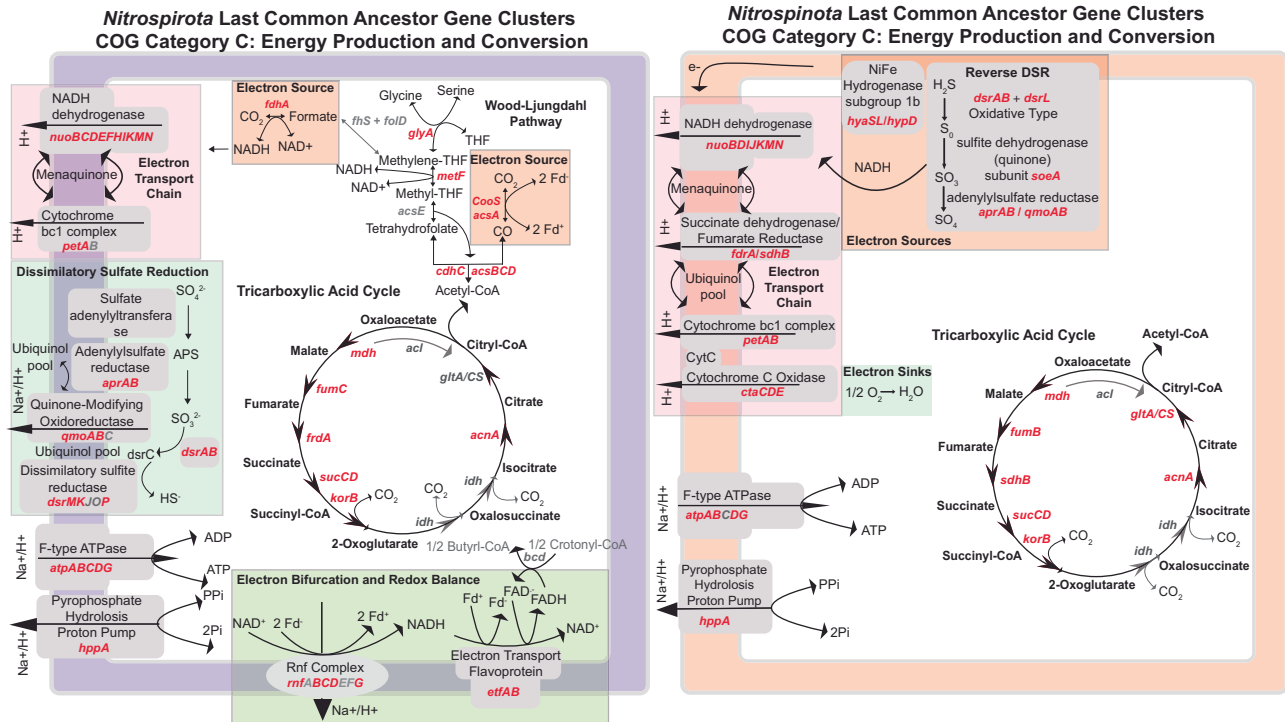
Fig. 4 Genome diagrams of COG Category C: Energy Production and Conservation gene clusters in putative last common ancestors (LCA) of Nitrospirota and Nitrospinota identified by ASR (0.5 > posterior probability) at the root node of the respective phylogenies. Gene symbols in red are present, gene symbols in gray are genes that are a part of the given pathway depicted, but are not present or are not above the 0.5 > pp threshold for inclusion in the LCA gene cluster set.
