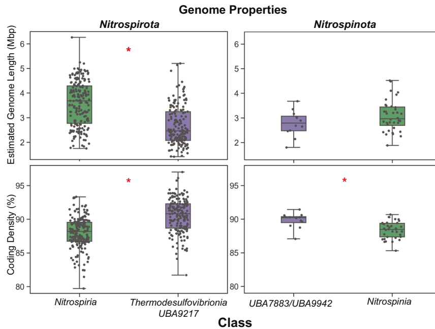
Fig. 2 Genome properties via CheckM of the major phylogenetic delineations (also corresponding to gene cluster content) in Nitrospirota and Nitrospina show that basal clades (purple) have smaller genome length and higher coding density than later branching clades (green). Estimated genome length y-axis scale is 10^6 base pairs, and coding density y-axis is as percent. Red asterisks denote results that show significant differences between metrics in the clades by a ANOVA ( p value < 0.05 ). For Nitrospirota the p values for genome length and coding density are 3.63e^{-20} and 3.25e^{-20} , respectively. For Nitrospina the p values for genome length and coding density are 0.13 and 0.0011, respectively.
