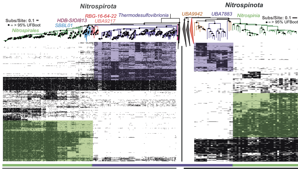
Fig. 1 Phylogenomic trees and gene content of Nitrospirota and Nitrospinota phyla, showing distinct clades and gene clusters associated with basal groups comprised mainly of subsurface organisms (purple bar at bottom) or later-branching groups (green bars at bottom). The trees are oriented so the middle of the image contains the outgroups for both trees. Phylogenetic trees were produced using the Bac120 marker set (min 12 genes) using the PhyloPhlan pipeline to create the alignments and IQ-TREE using the LG + F + G4 model chosen by ModelFinder using the Bayesian Information Criterion (BIC) and 1000 ultra-fast non-parametric bootstraps. Heatmaps of gene cluster absence (empty) or present in at least 10% of the genomes in the given phyla (filled) are displayed below the trees. Rows of gene clusters are ordered by hierarchical clustering using wards linkage. Blocks of genes enriched in the Nitrospina or Nitrospira are highlighted with the green boxes, and purple used to highlight the enriched gene clusters in the basal classes of the given phyla. Hierarchical clustering of genomes solely by gene content produced similar groupings as the phylogenies (Supplementary Figure 5).
