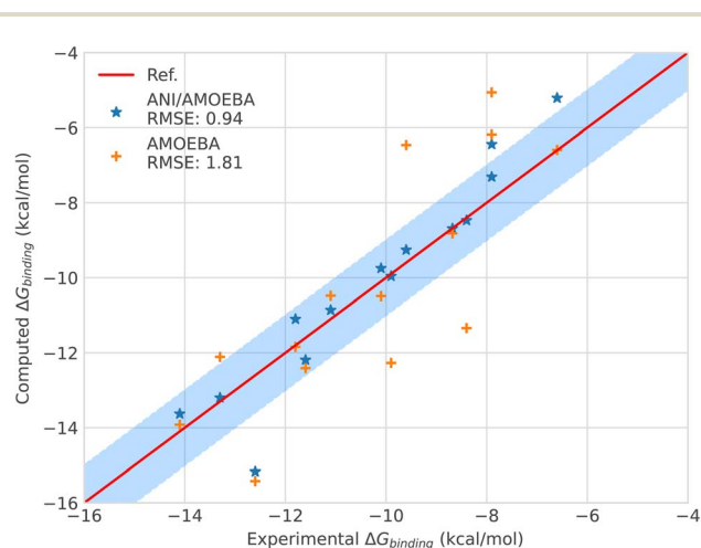
Fig. 3 Binding free energies of host–guest systems of the SAMPL4 and SAMPL6 blind challenges with AMOEBA (orange) from ref. 78 versus hybrid model ANI-2X/AMOEBA (blue) and experimental (red). The blue domain corresponds to the so-called chemical accuracy: error of 1 \text{ kcal mol}^{-1} w.r.t. experiment.
