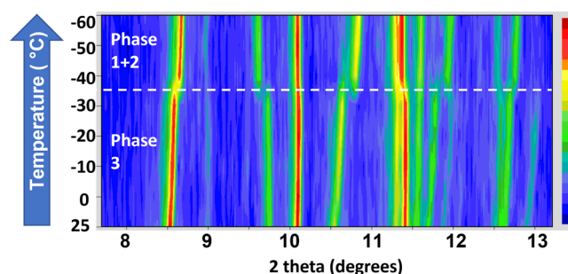
Figure 1. Contour plot of VT-PXRD data collected on [\text{H}_3\text{N}(\text{CH}_2)_6\text{NH}_3]\text{PbBr}_4 between room temperature and -60 °C. Note that data were collected using Mo K\alpha_1 radiation and the y -axis is not linear.
