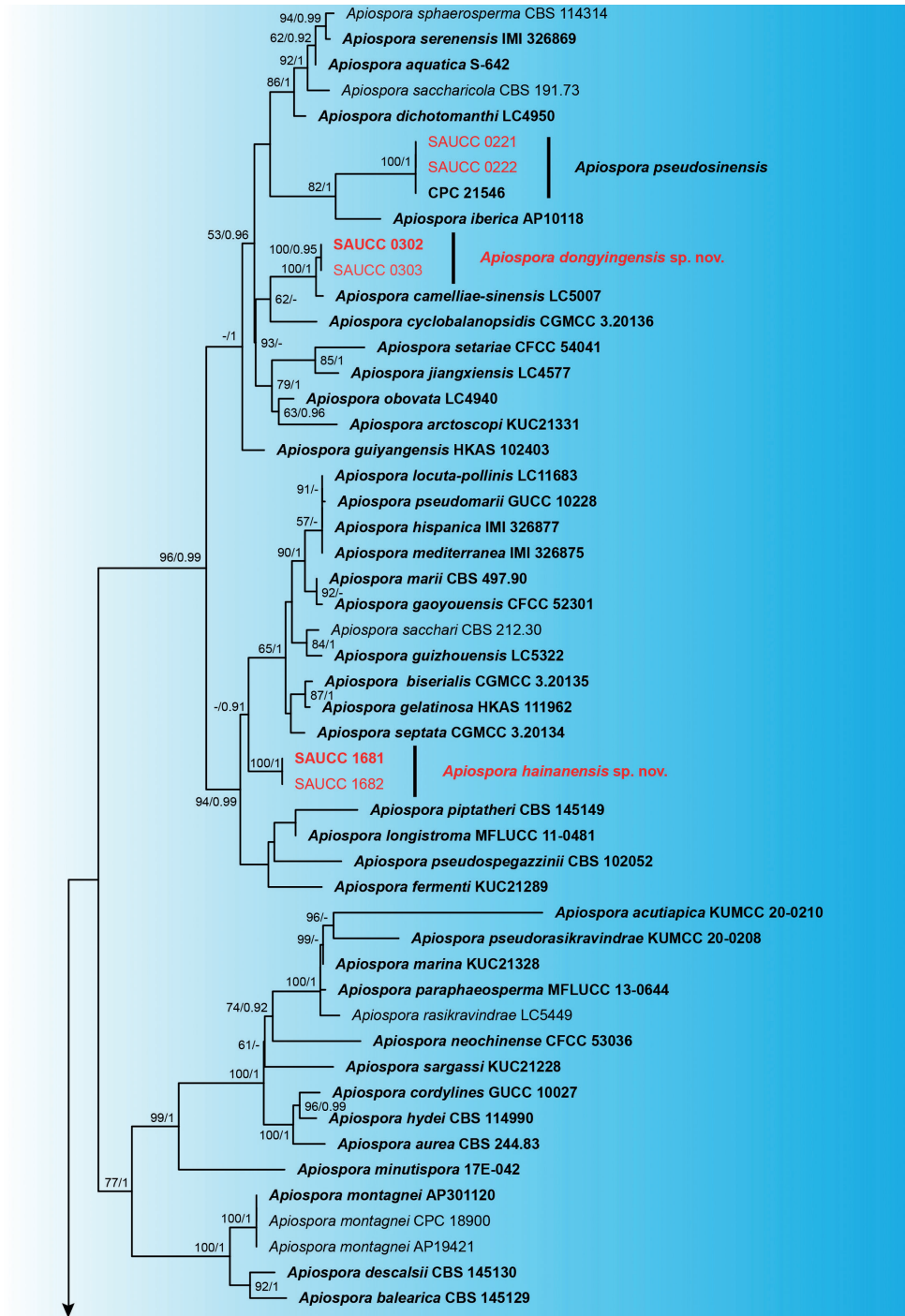
Figure 1. Phylogram of Apiospora based on combined ITS, LSU, tef1 and tub2 genes. ML bootstrap support values (MLBS \geq 50%) and Bayesian posterior probability (BYPP \geq 0.90) are shown as first and second position above nodes, respectively. Strains from this study are shown in red, ex-type or ex-epitype cultures are indicated in bold face. Some branches were shortened according to the indicated multipliers.
