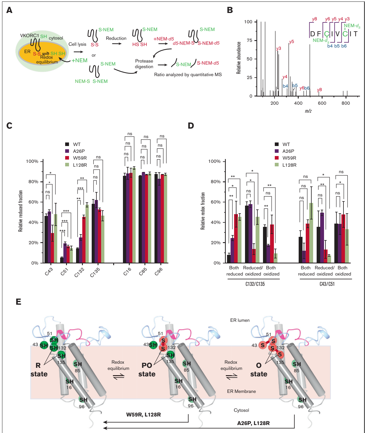
Figure 3. MS-based footprinting reveals that severe WR mutants induce the shift of the VKOR active site to an aberrantly reduced state. (A) Scheme of MS-based footprinting. VKOR cysteines located in the ER are in equilibrium between oxidized and reduced states, and those in the cytosol or inside the ER membrane remain reduced. The membrane permeable NEM (ie, NEM- d_0 ) is used to label all reduced cysteines in cells. After cell lysis, the oxidized cysteines are subsequently reduced by tris(2-carboxyethyl) phosphine hydrochloride (TCEP), labeled by the NEM- d_5 isotopologue, resulting in a mixture of d_0 and d_5 proteins, and digested. MS quantification to provide the ratio of the isotopically labeled peptides gives the redox state of each cysteine in the cells. (B) Representative product-ion (MS/MS) spectrum of a peptide with both Cys12 and Cys13 labeled by NEM- d_5 . (C) Relative reduced levels of cysteines in WT VKOR and severe WR mutants. All 3 severe WR mutants shift Cys51 and Cys132 to an aberrantly reduced state. As controls, Cys16 (TM1), Cys85 (TM2), and Cys96 (cytosolic loop) remain in the reduced state in WT and mutants. The error bars are from 3 different peptides and two-tailed student t test are used. * P < .05 , ** P < .01 , *** P < .001 . (D) Relative redox fractions of cysteine pairs. The severe WR mutants shift Cys132/Cys135 at the active site to an aberrantly reduced state. (E) Structural interpretation of MS detected the state of VKOR cysteines. Severe WR mutants shift the cellular state of Cys132/Cys135 from PO or O state to R state. WT, wild-type.
