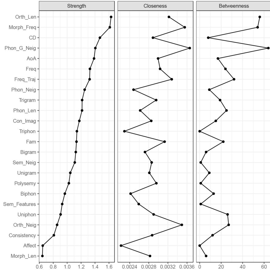
Figure 6. Three centrality indices of the psychometric network model over 1,728 words: strength, closeness and betweenness. Strength refers to the sum of absolute partial correlation values for each node. Closeness refers to the inverse of the sum of distances from one node in the network to all other nodes. Betweenness refers to the number of the shortest paths that one node was passed through. The variables are ordered in an ascending order by strength.
