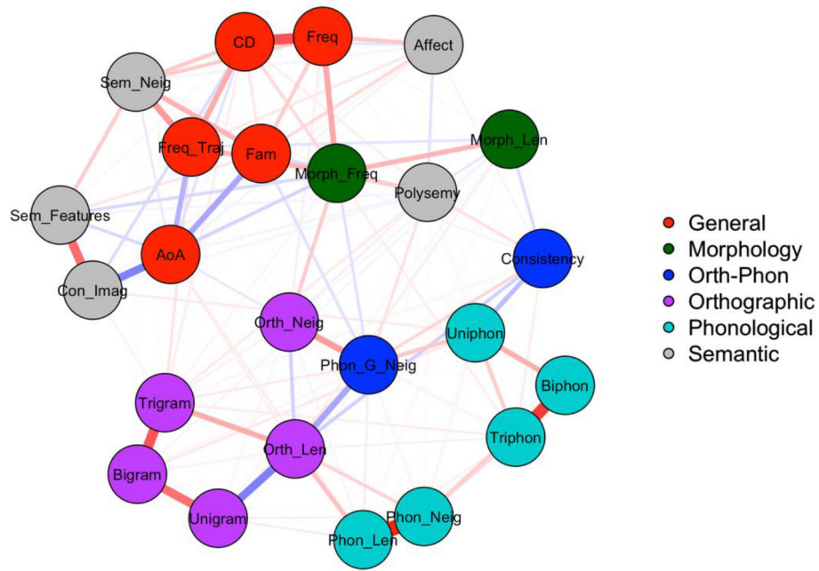
Figure 5. Psychometric network model describing relationships between independent variables over 1,728 words. Line thickness refers to the edge strength, which is the size of the partial correlation between variables. Line colors indicate the sign of the correlation, in which red lines correspond to a positive correlation while blue lines correspond to a negative correlation.
