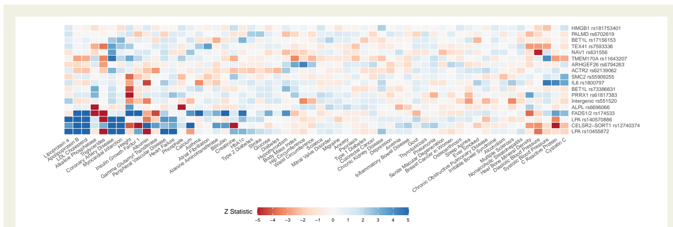
Figure 3 Association of aortic stenosis variants with biomarkers, physiological measurements, and diseases. Variants were ordered to reflect similarity in their associations with traits and vice versa. The strength and direction of associations are represented by cells of different colors, with blue cells indicating positive effects on the odds of aortic stenosis and red cells indicating inverse associations. For ease of visualization, Z statistics >5 or less than -5 were rounded to 5 and -5, respectively.
