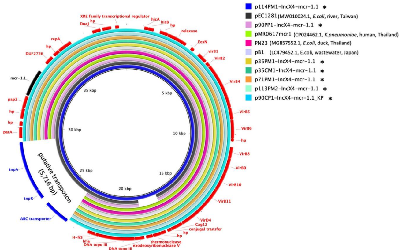
Figure 4. Circular alignments of IncX4/ mcr-1 complete plasmids. Alignment of mcr-1 /IncX4 complete plasmids in this study (marked with asterisk*) with plasmid sequences from Genbank: pEC1281 (accession no. MW010024.1), pMR0617mcr1 (accession no. CP024462.1), PN23 (accession no. MG857552.1) and pB1 (accession no. LC479452.1). The innermost circle represents the main reference sequence in the alignment. ARGs and mobile genetic elements are labelled in the outermost circle.
