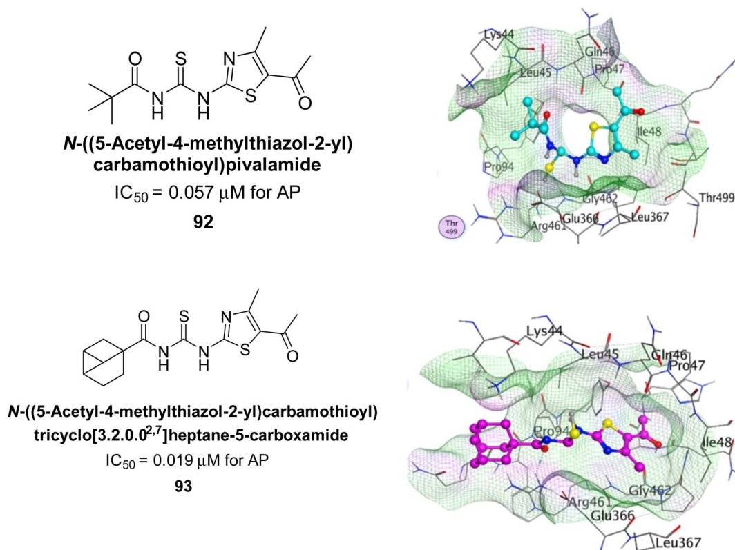
Fig. 37 Chemical structures of compounds 92 and 93 and their AP inhibition.
