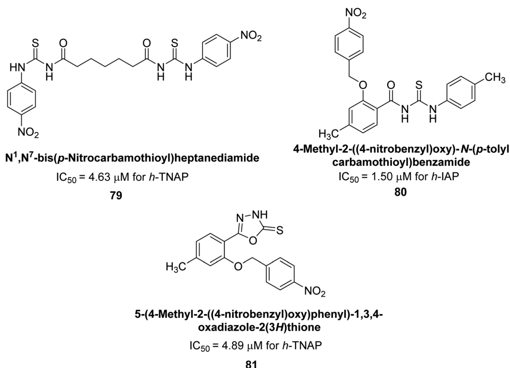
Fig. 30 Chemical structures of compounds 79, 80 and 81 and their TNAP and IAP inhibitions.
