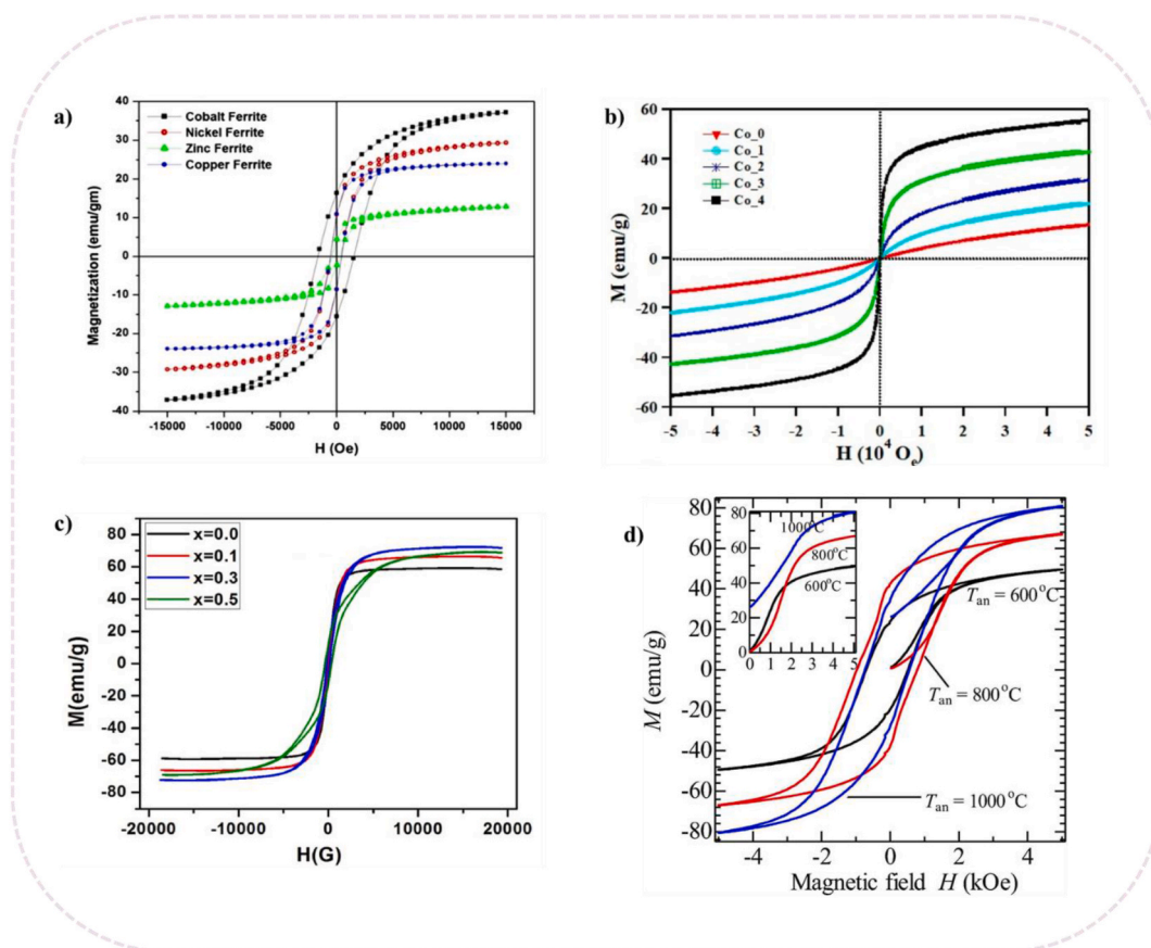
Fig. 2. Magnetization-field ( M – H ) typical hysteresis curves. a) MFe_2O_4 ( M = Zn, Ni, Cu, and Co ) [54], b) Co_2Zn_{1-x}Fe_2O_4 ferrite [55], c) Li_{0.25}Mn_{0.5-x}Co_xFe_{2.25}O_4 [56] and d) Co-precipitated CoFe_2O_4 nanoparticles at various calcination temperatures (600 °C, 800 °C and 1000 °C) [57].
