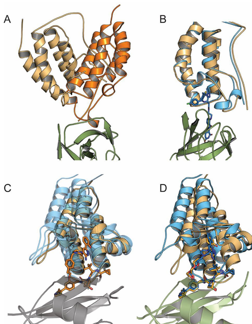
Figure 4. Models of CRBN–dBET57– BRD4BD1 and VHL- PROTAC1/2-SMARCA2/4 complexes. (A) Superposing the best model (model 5) of CRBN–dBET57– BRD4 BD1 (light orange) and the consensus prediction of CRBN–dBET23– BRD4 BD1 (bright orange) to show that they substantially differ. (B) Model 5 of CRBN–dBET57– BRD4 BD1 (blue), superimposed on its X-ray structure (orange, PDB ID: 6BNB). (C) Superimposing the best model (model 2) of VHL- PROTAC2-SMARCA2 (orange) at the center of the consensus cluster and the consensus models of VHL- PROTAC1-SMARCA2 and VHL- PROTAC2-SMARCA4, both shown in transparent blue color. (D) Superimposing the consensus prediction (model 5) of VHL- PROTAC1-SMARCA2 (blue) and its X-ray structure (orange, PDB ID: 5NVX)
