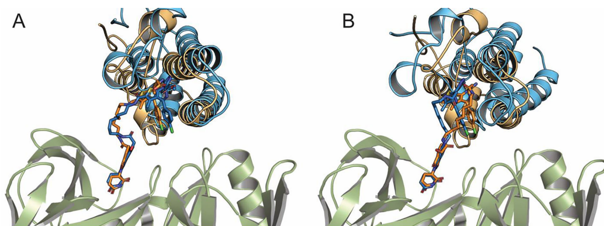
Figure 2. Accuracy of some predicted structures. (A) Model 3 of the CRBN-dBET23-BRD4 BD1 complex (blue), superimposed on its X-ray structure (orange, PDB ID: 6BN7). (B) Model 5 of the CRBN-dBET6-BRD4 BD1 complex (blue), superimposed on its X-ray structure (orange, PDB ID: 6BOY)
