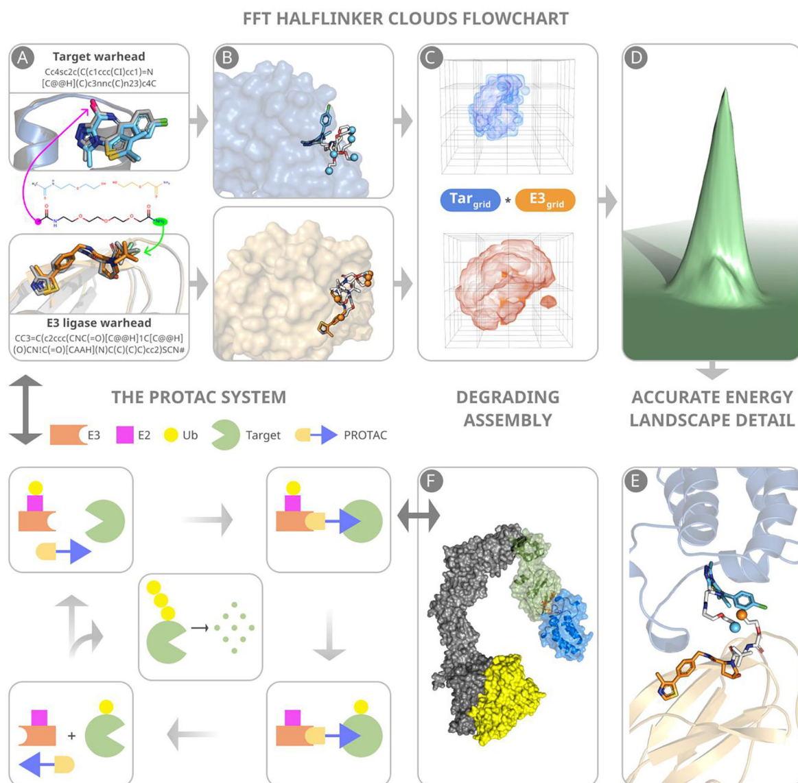
Figure 1. Main steps of predicting PROTAC structures. (A) Warheads are docked to component proteins. Green and magenta arrows indicate attachment points to the E3 ligase and target warheads, respectively. (B) Half-linker conformations are generated and attached to each protein-bound warhead. The small colored spheres represent the half-linker end points. In the VHL:MZ1:BRD4BD2 (PDB ID: 5T35) complex shown, the BRD4 warhead and the end points of the attached half-linkers are depicted in cyan, and the VHL warhead and the end points of the attached half-linkers are in orange. (C) Generating favorable protein-protein poses that have half-linker ends placed sufficiently close to each other. (D) Selection of low energy poses. (E) A resulting pose with half-linker end points in close proximity before connecting the half-linkers. (F) The VHL–ElonginC–ElonginB–Cul2–Rbx1 structural assembly with the CRL2VHL complex shown in blue. The assembly includes a ubiquitin-like protein (ULP), shown in yellow, separated by a favorable distance to facilitate transfer
