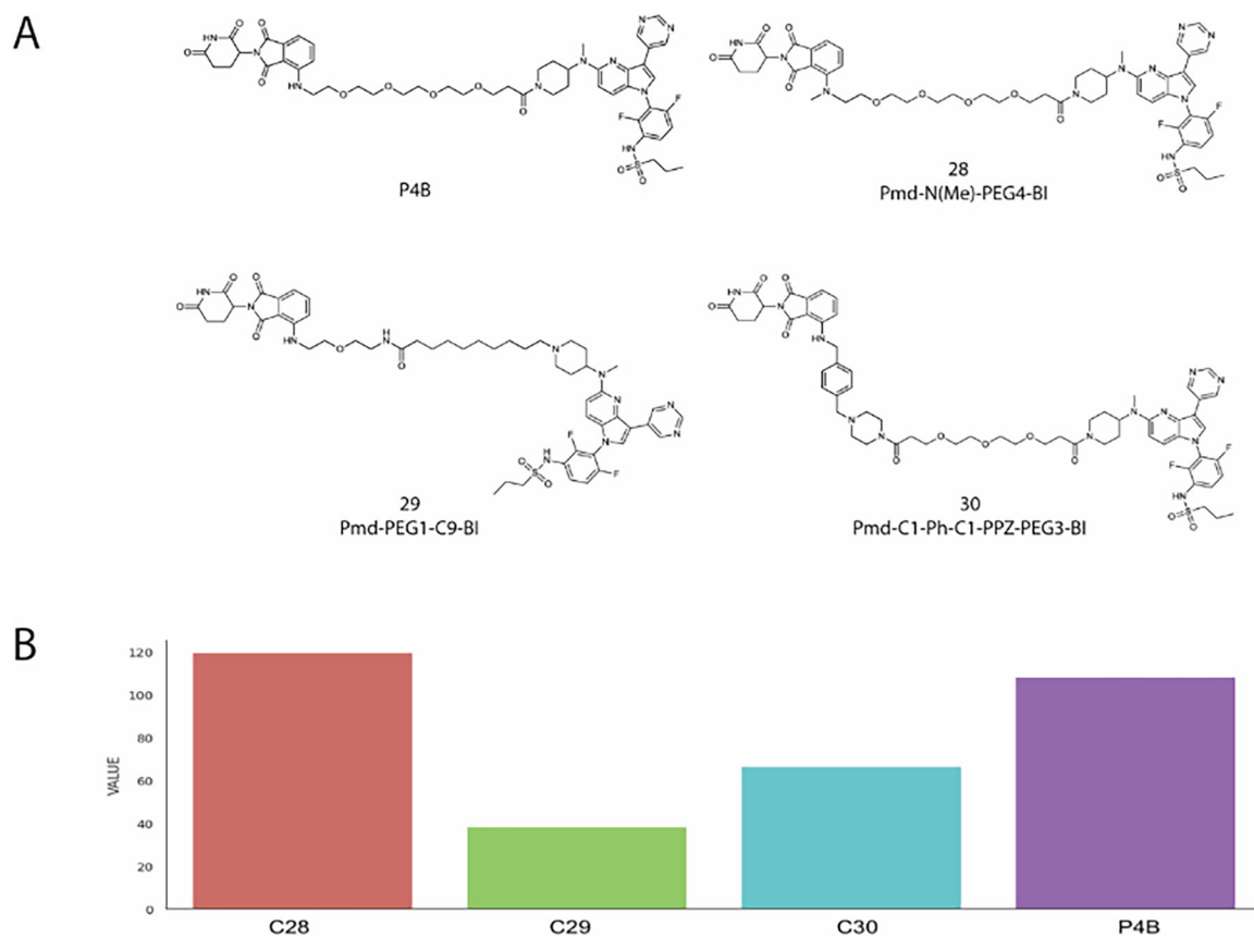
Figure 6. In cell BRAF degradation analysis. (A) Chemical structures of P4B and compounds 28–30. (B) Relative degrading activity of PROTACs 28, 29 and 30 and P4B as predicted using our computational method. Value is the weighted number of predicted structures that satisfy the restraints posed by the linker, considered as the prediction of degrading activity.
