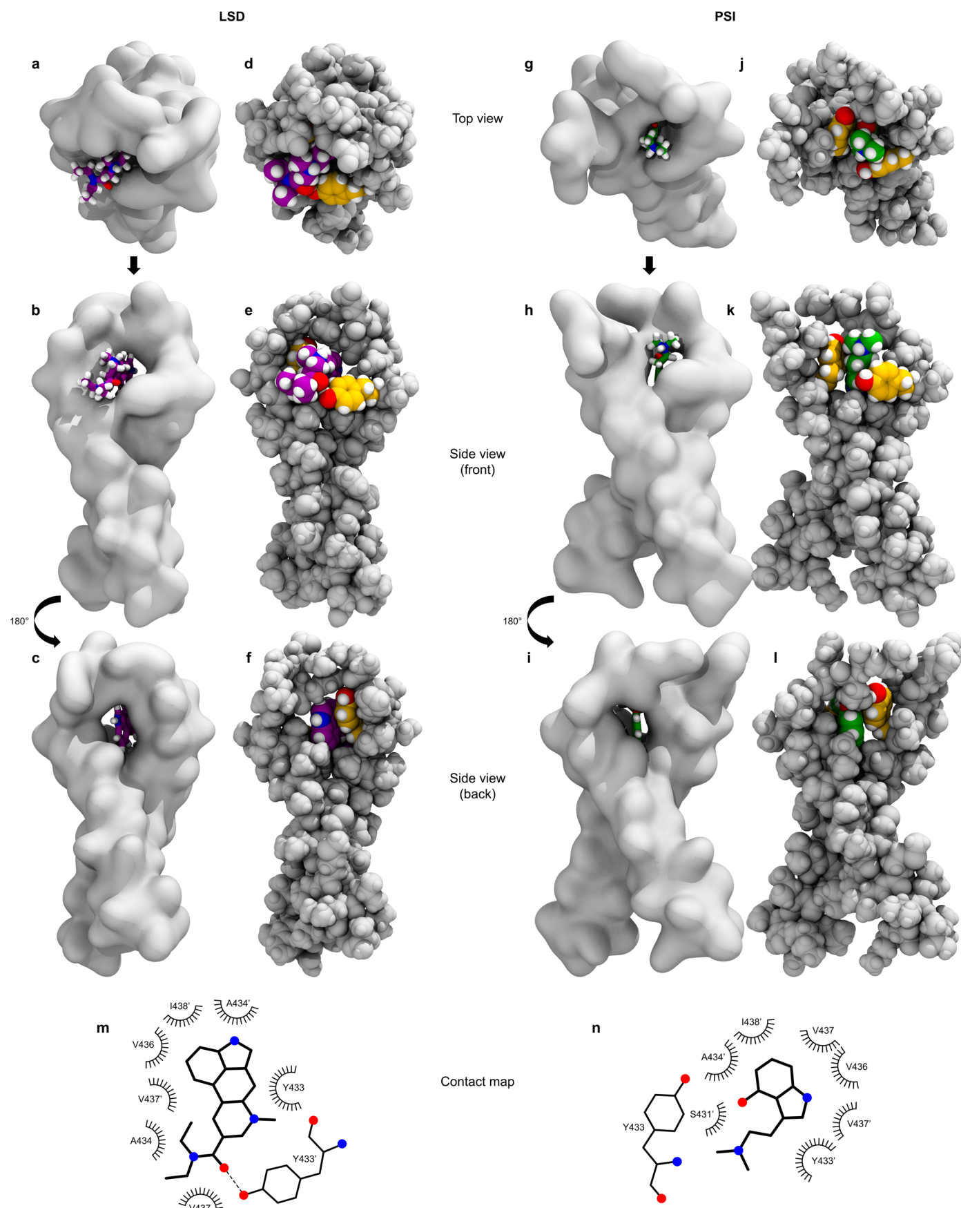
Extended Data Fig. 3 | Representative atomistic MD snapshots showing the binding pocket for LSD + (purple) and PSI + (green) in the extracellular-facing crevice of the wild-type TrkB TMD dimer (gray). a-c, g-i, Drugs are shown in licorice representation and protein is shown in surface representation. d-f, j-l,
