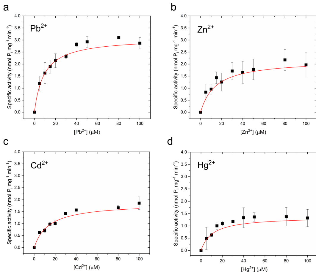
Fig. 4 M^{2+} -dependent CmΔZntA ATPase activity in proteoliposomes. (a) Pb^{2+} -dependent, (b) Zn^{2+} -dependent (c) Cd^{2+} -dependent and (d) Hg^{2+} -dependent specific ATPase activity as a function of metal concentrations (0–100 μM). Data were fitted with a Michaelis–Menten-like equation as described in Materials and methods. All the ATPase activity measurements were corrected for background values for control liposomes and all data are mean \pm s.d. ( n = 3 ).
