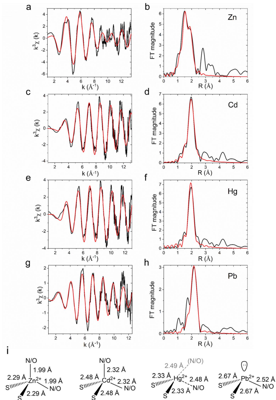
Fig. 5 X-ray absorption spectroscopic analysis (XAS) of Cm ΔZntA- M^{2+} . K-edge experimental EXAFS data (black line) and the best fit (red line), with corresponding Fourier transforms, of Cm ΔZntA- Zn^{2+} (a and b) and Cm ΔZntA- Cd^{2+} (c and d); L_3 -edge EXAFS data and corresponding Fourier transforms for Cm ΔZntA- Hg^{2+} (e and f) and Cm ΔZntA- Pb^{2+} (g and h; for details on data collection and analysis see the Material and methods section). Parameters for the fits are reported in Table 2. (i) Models of the coordination geometries and metal–ligand bond distances for Cm ΔZntA- Zn^{2+} , Cm ΔZntA- Cd^{2+} , Cm ΔZntA- Hg^{2+} and Cm ΔZntA- Pb^{2+} .
