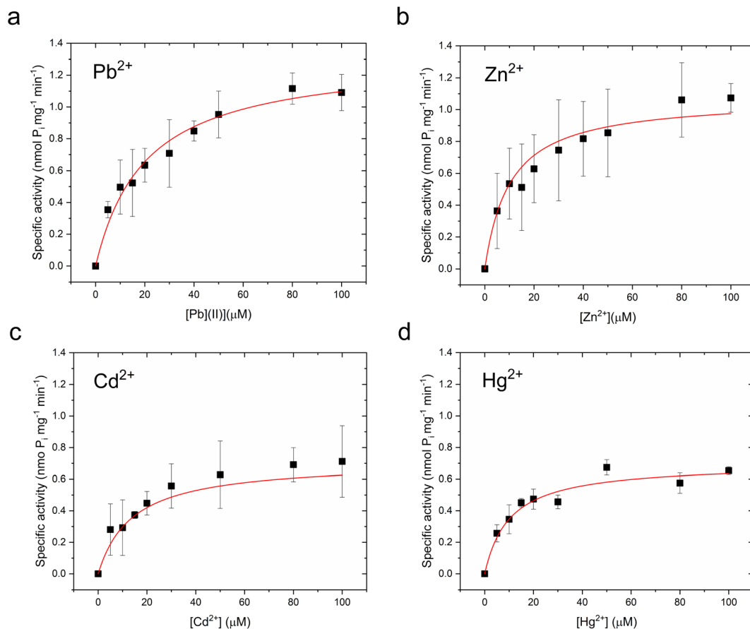
Fig. 3 M^{2+} -dependent CmΔZntA ATPase activity in Cymal-7 micelles. (a) Pb^{2+} -dependent, (b) Zn^{2+} -dependent, (c) Cd^{2+} dependent, and (d) Hg^{2+} -dependent specific ATPase activity, as a function of metal concentration (0–100 \mu M ). Data were fitted with a Michaelis–Menten-like equation as described in Materials and methods. All the ATPase activity measurements were corrected for the background ATPase activities obtained with control samples without Mg^{2+} , required as cofactor for ATP binding and hydrolysis. All data are mean \pm s.d. ( n = 3 ).
