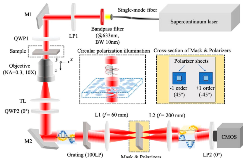
Figure 1. System design of polarized shearing interference microscopy. LP1 and LP2, linear polarizers; M1 and M2, mirrors; QWP1 and QWP2, quarter wave plates; TL, tube lens; L1 and L2, lenses. The z -axis is the direction of the optical axis, and the x - y plane is the sample plane. The zoomed region denotes the circular polarization illumination and the location of the masks and polarizer sheets on the Fourier plane. After QWP2, the laser beams' polarization directions are shown with cartoon insets in the beams.
