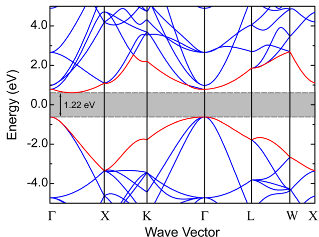
Fig. 2 Electronic band structure of unstrained BiAs bulk crystal. Notice the 1.22 eV indirect gap between the \Gamma and X directions of the first Brillouin zone.
