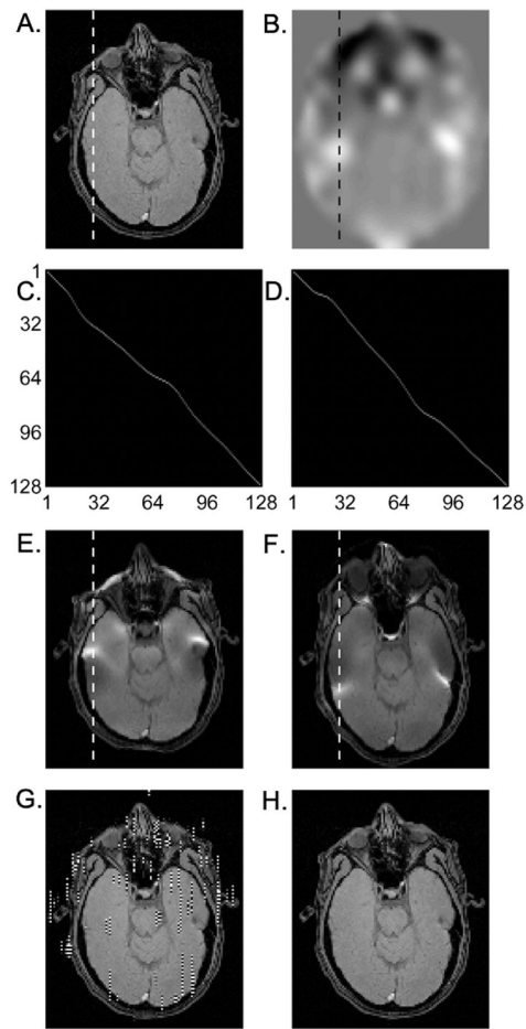
Figure 8: Illustration of EPI distortion correction using Eq. (14).
