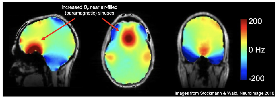
Figure 2: B_0 magnetic field in the brain at 7T with 2 nd order shimming.
