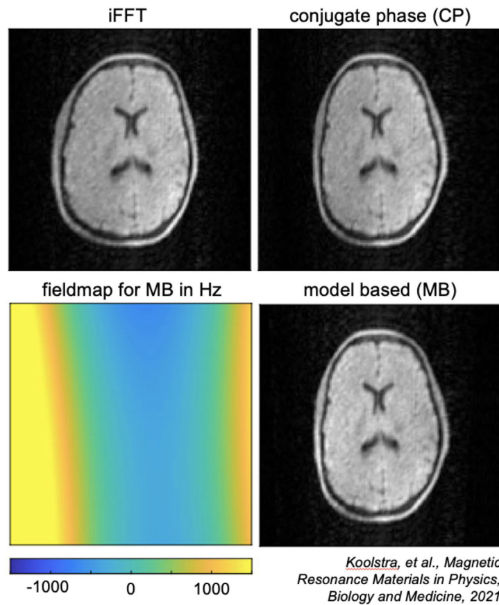
Figure 9: CP and MB reconstruction at 50mT.
