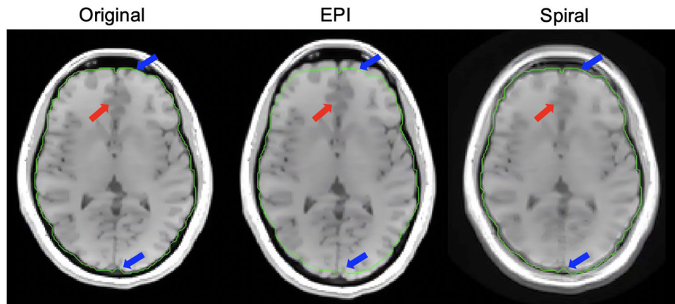
Figure 6: Image simulations: Cartesian vs. non-Cartesian.
