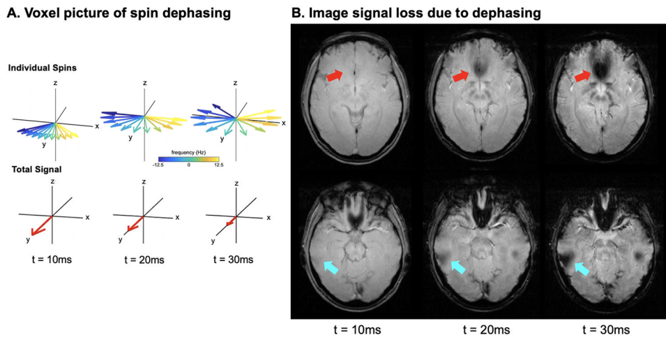
Figure 4: Signal Loss from Spin Dephasing.
