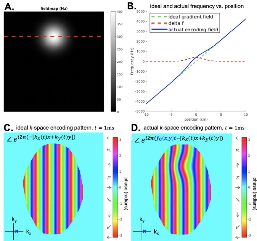
Figure 5: Ideal vs. actual encoding phase at a single k-space location.
