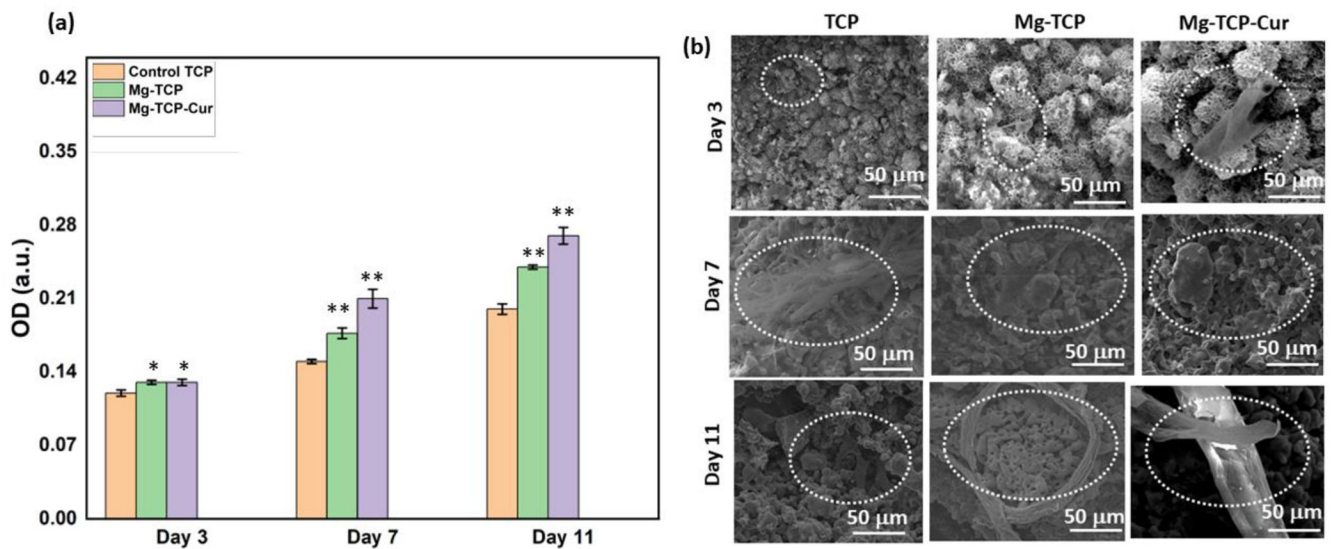
Fig. 2: Interactions of osteoblast with 3D printed scaffolds (a) MTT assay results show that the tested compositions are cytocompatible. On day 3, Mg-TCP and Mg-TCP-Cur show slightly higher cellular viability than the control. On day 7 and day 11, the treatment samples indicate significantly enhanced cell viability than the control. The Mg-TCP sample shows ~ 1.2 times enhancement, the Mg-TCP-Cur shows ~ 1.4 times enhancement than the control. In the image, * indicates a p-value of <0.05 and the ** denotes a p-value of <0.0001 (b) Good cellular attachment on each sample surface is seen in the FESEM images. The treatment samples show the presence of extended filopodial attachment. The observed cells and extended filopodia are marked with the dotted circle in the images.
