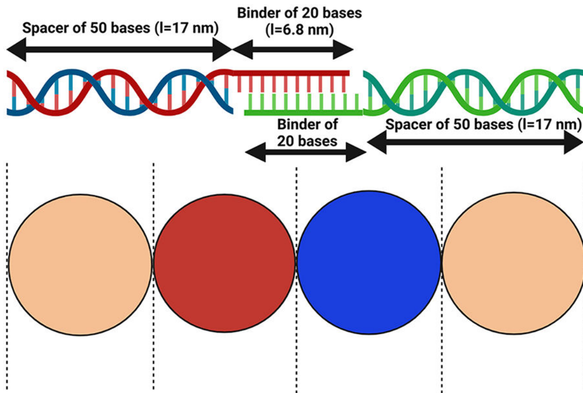
Fig. A3. Complementary binders in our CG model mapped onto the dsDNA and ssDNA configuration of Ref. 23 for scale. Complementary outer binder particles (red and blue) form a dynamic bond representing the interaction between complementary DNA strands (Figure created with https://biorender.com/ ).
